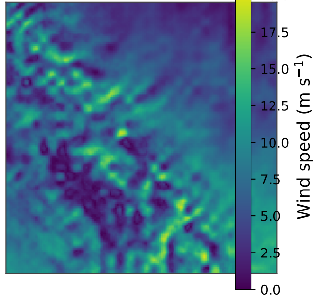
Topology-inspired
