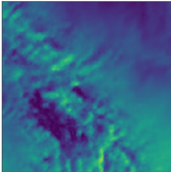
Pretrained CNN
