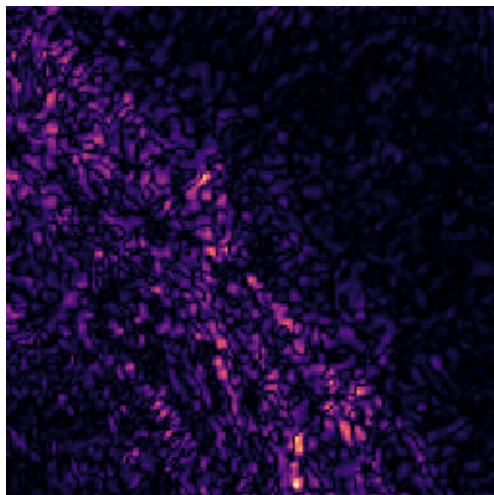
|CNN – GT|
