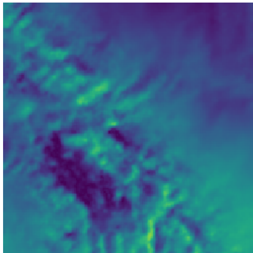
Pretrained CNN
