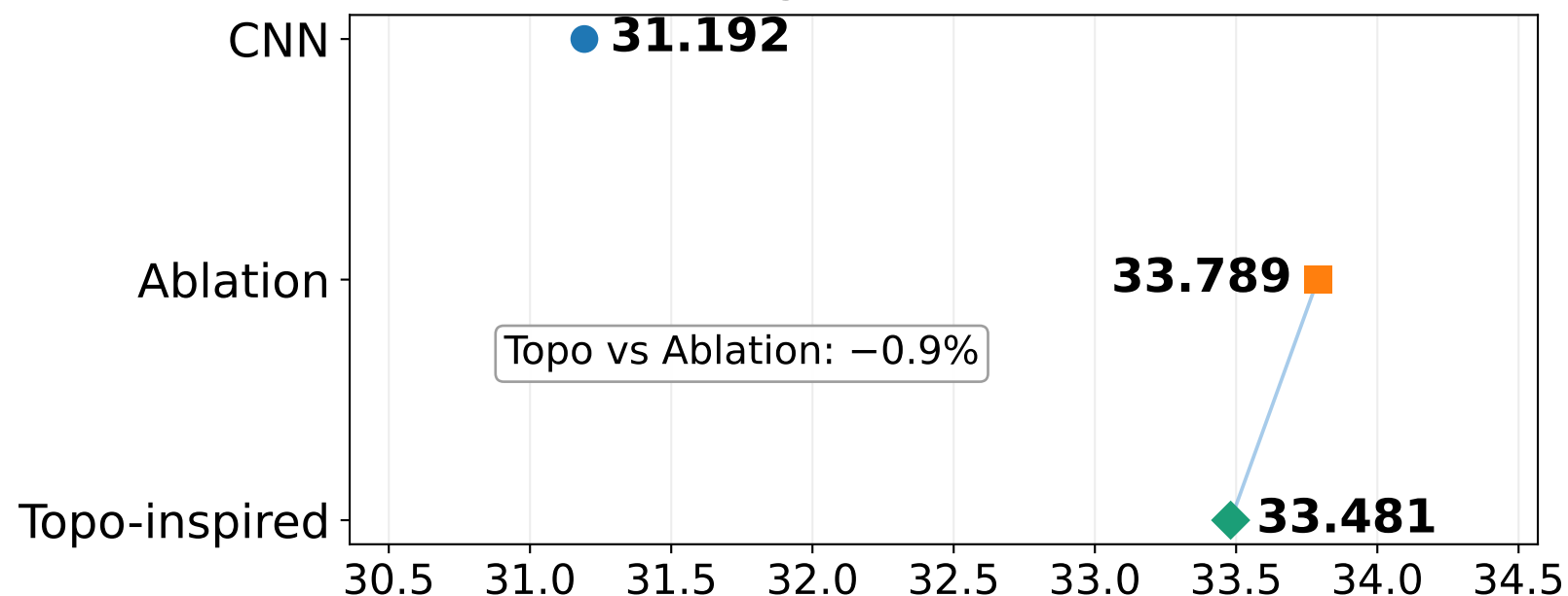
PSNR uv (higher is better)
