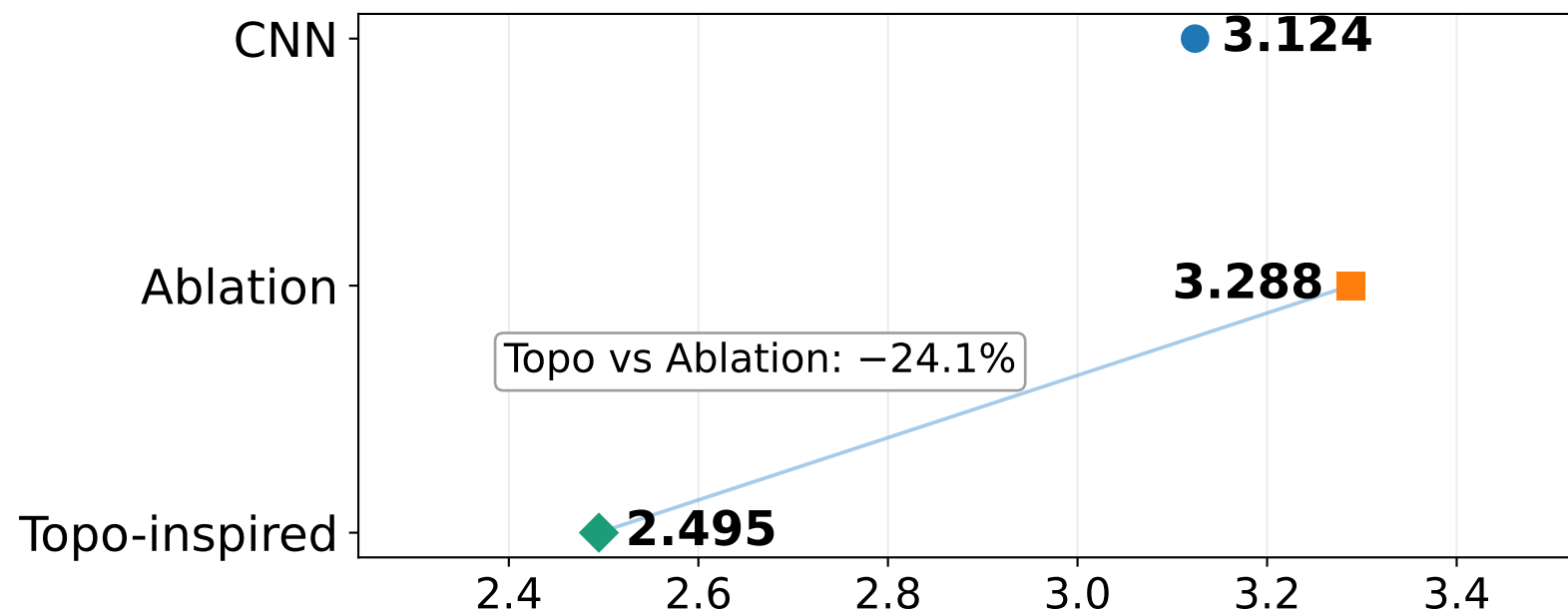
Bottleneck d_B (lower is better)
