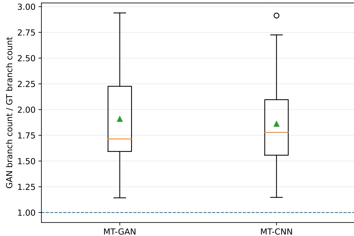
Does MT-GAN have lower GAN over-fragmentation?
