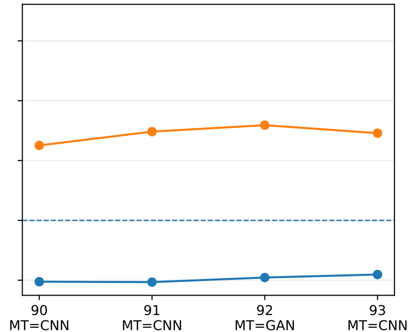
Adjacent cluster 90-93
