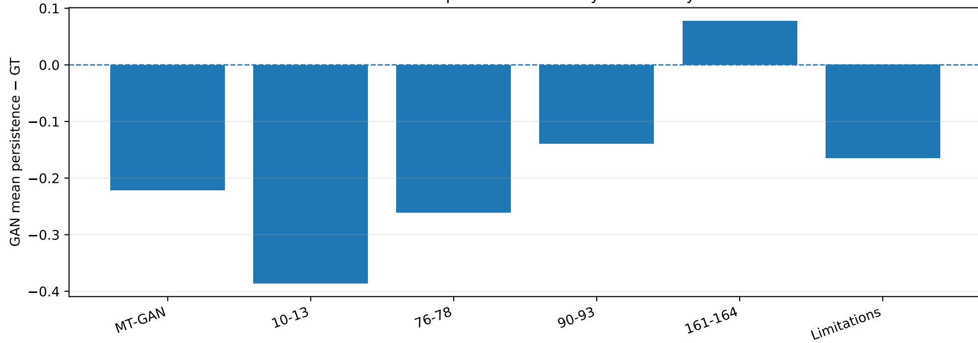
GAN mean-persistence bias by case family
