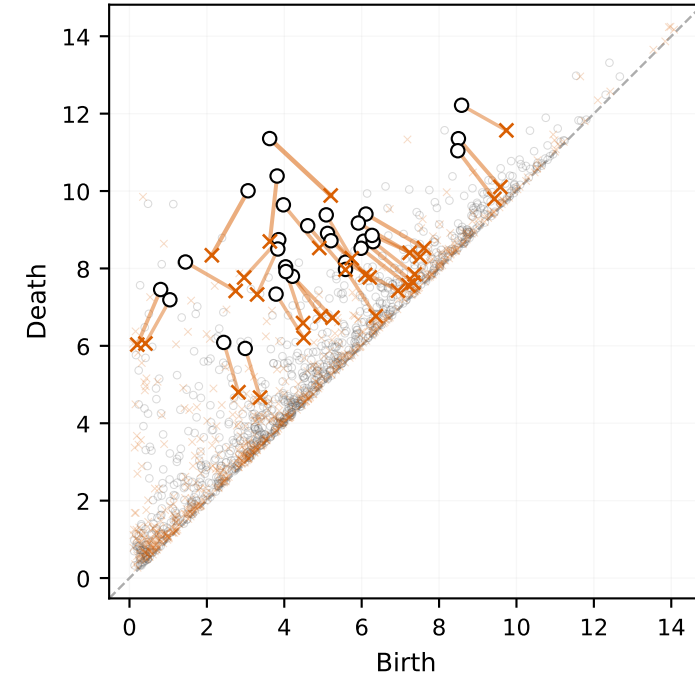
Candidate F vs GT — D_1
