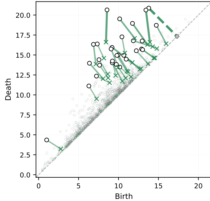
Ablation ( L_{UV} only) vs GT — D_1
