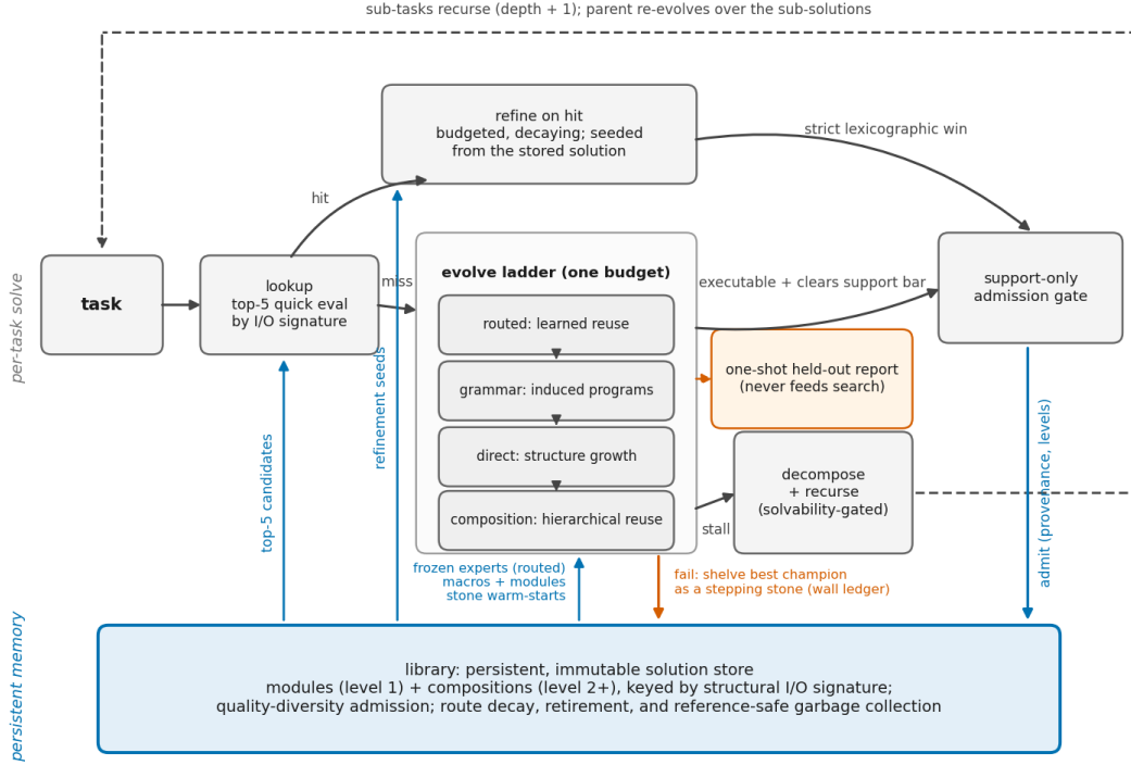
Figure 1: The Versal task loop. Search begins from persistent memory, escalates through reuse and structural search, may recurse over typed subtasks, and returns verified artifacts to a lifecycle-managed library. Held-out query evaluation occurs only after search selects an executable artifact.
