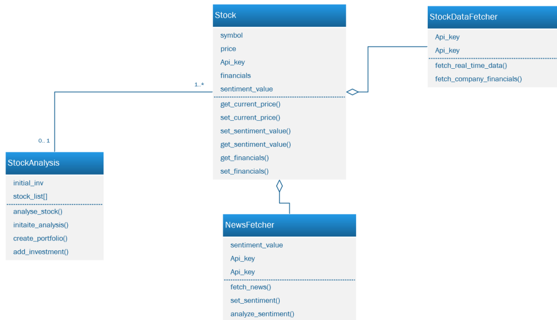
Structural Class Diagram
