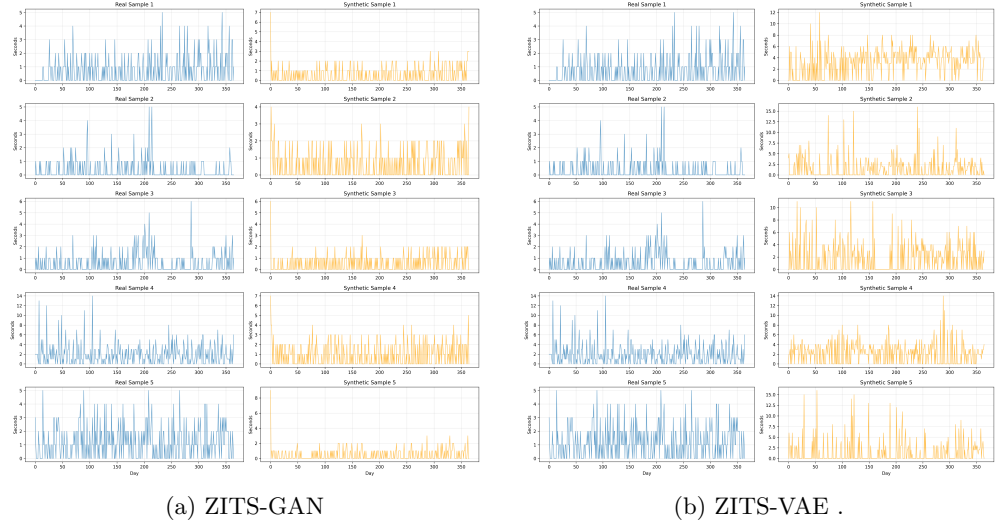
Fig. 2: Real (blue) and synthetically generated (orange) examples of the (a) ZITS-GAN and (b) ZITS-VAE proposed models for the M5 dataset.
