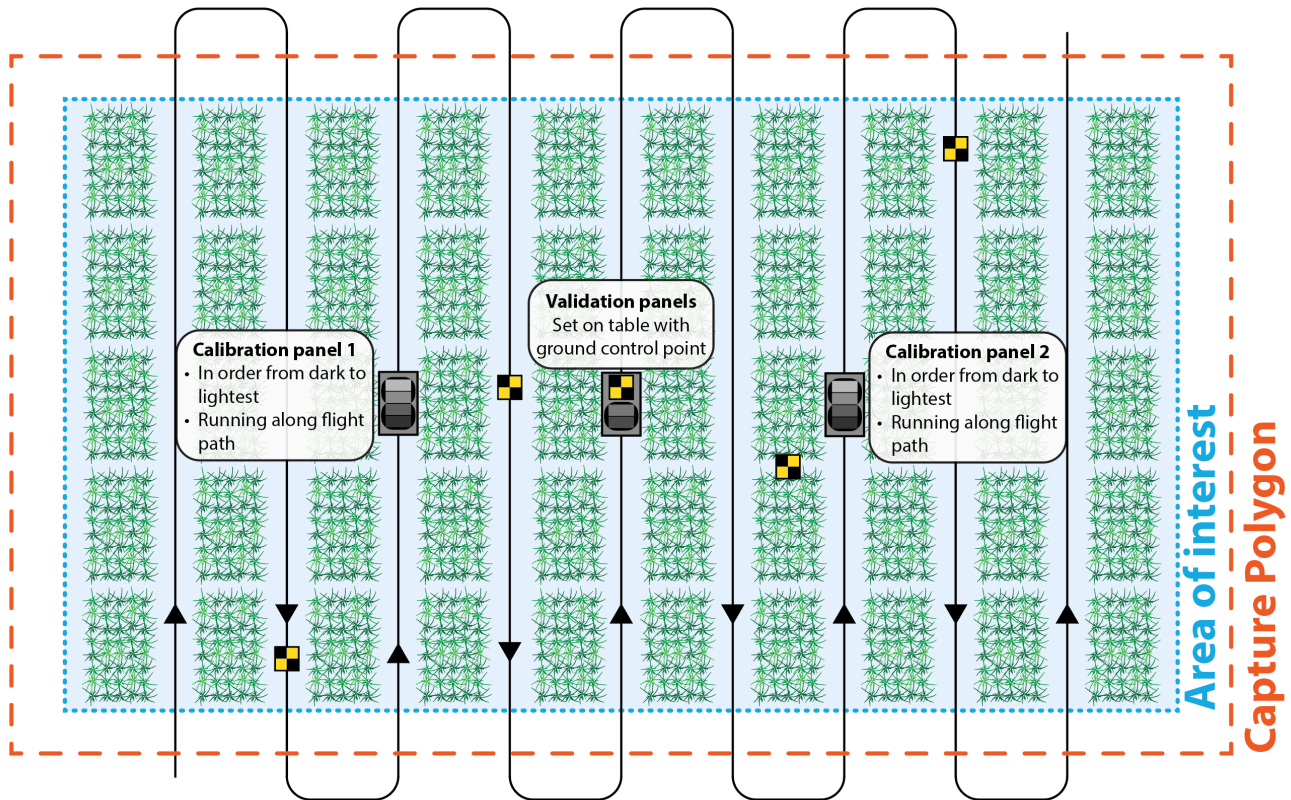
Figure: Dual ELM panel flight layout — default layout for CALViS surveys. See the Dual ELM panel flight section of the Standard Flight Procedure for the full rationale and alternative layouts.
