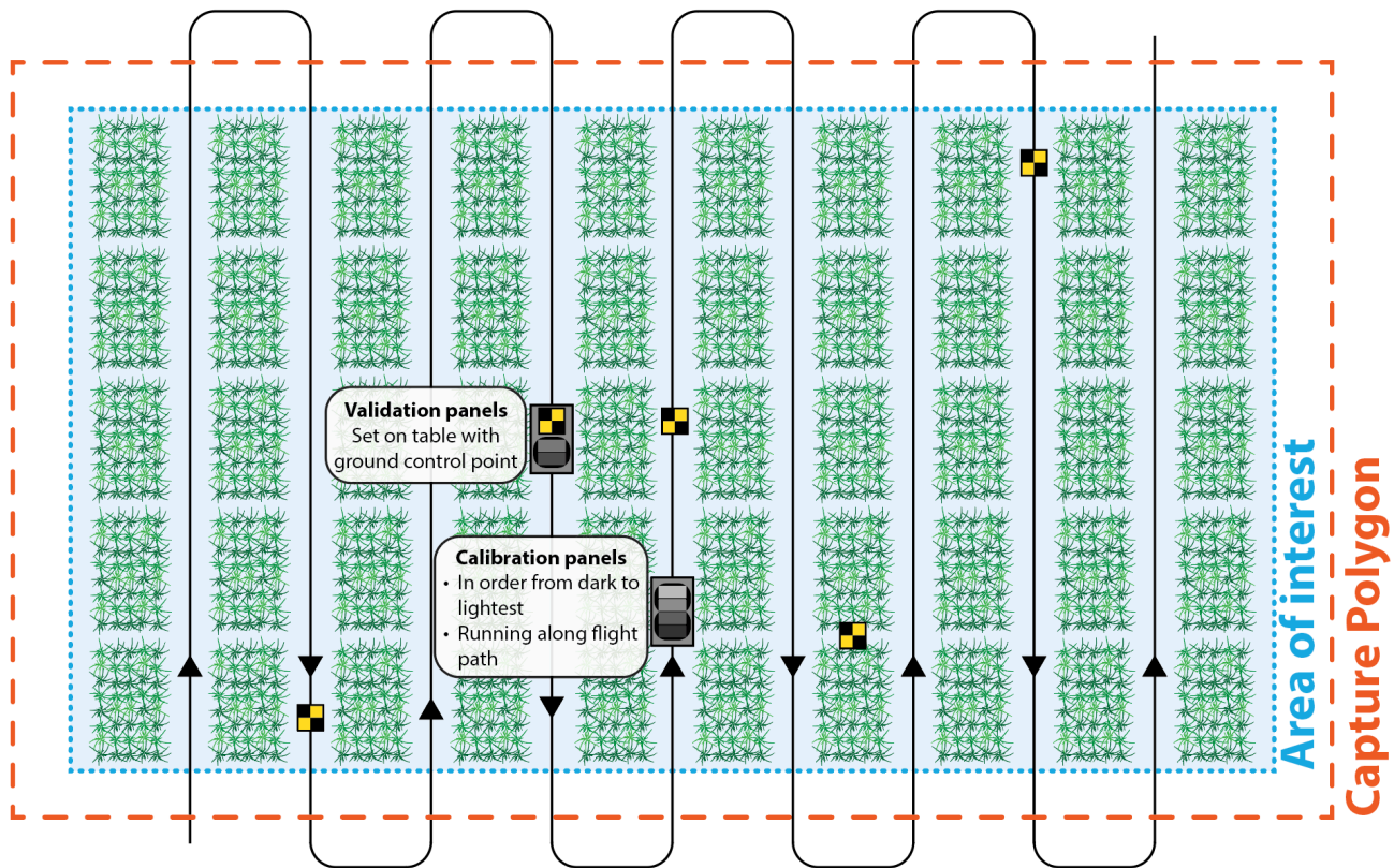
Figure: Single ELM panel flight layout. One 4-panel reflectance set is deployed near the centre of the survey area, alongside the validation panel set and its paired GCPs. The 5-GCP layout covers centre, corner, and off-axis positions, and all panels and GCPs sit inside the ~10% effective capture area inset from the polygon edge.
