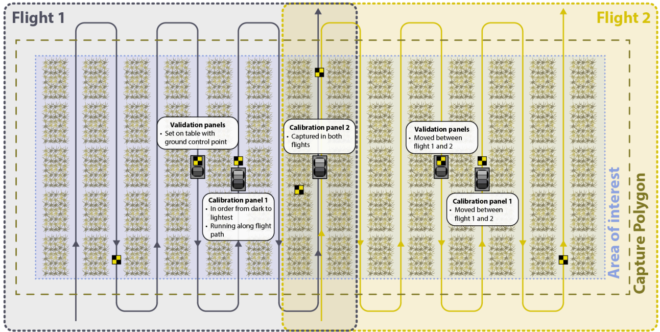
Figure: Multi-Flight Capture layout. The survey area is split into two sub-flights with a deliberate overlap zone at their shared boundary. A shared ELM panel set and two tie GCPs sit inside the overlap (and are left in place between sub-flights), giving both sub-flights a common radiometric and geometric anchor. Each sub-flight otherwise follows the dual-panel layout, with the validation panel set in one sub-flight and an expanded GCP distribution across the full area.
