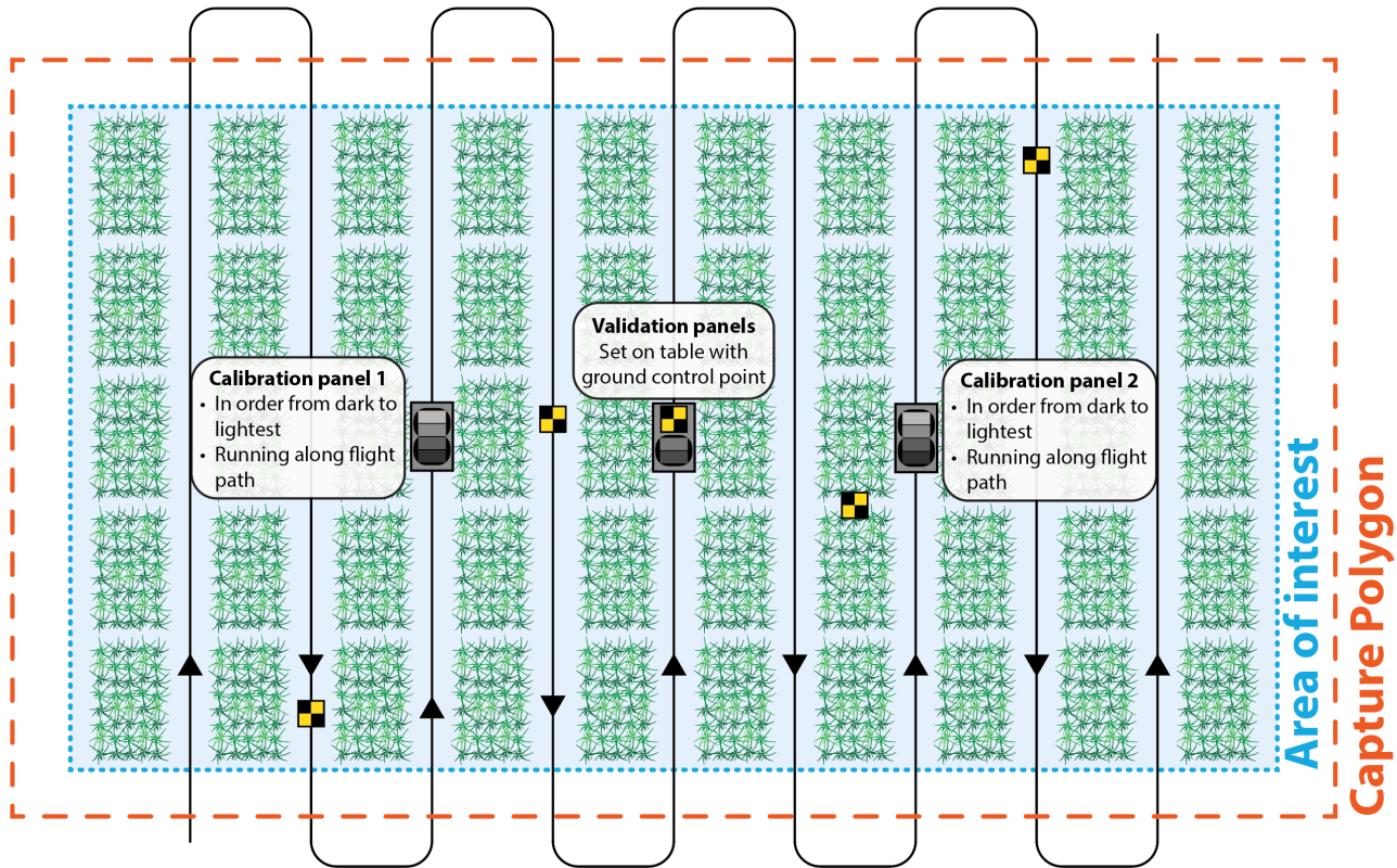
Figure: Dual ELM panel flight layout. Two reflectance panel sets are deployed at approximately the 1/3 and 2/3 positions along the long axis of the survey area, with the validation panel set and its paired GCPs near the centre. The 5-GCP layout covers centre, corner, and off-axis positions, and all panels and GCPs sit inside the ~10% effective capture area inset from the polygon edge.
