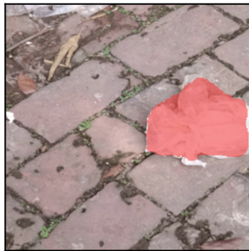
DeepLabV3+ mIoU 0.72
