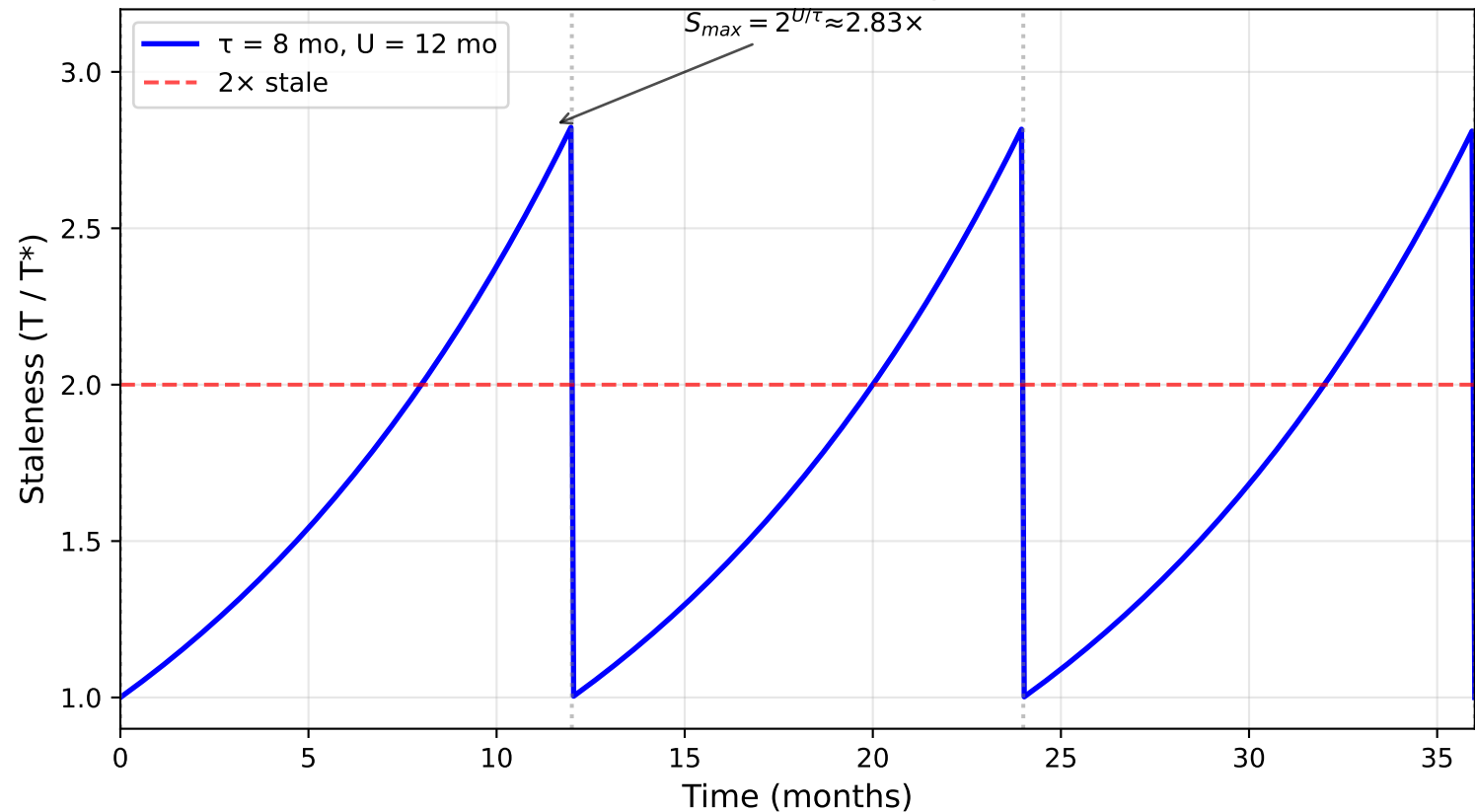
Policy Threshold Staleness Over Time ( \tau = 8 months, annual updates)
