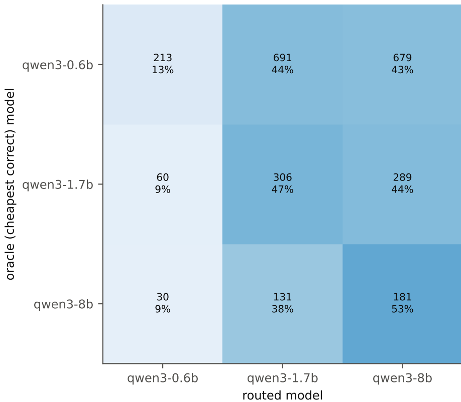
Router confusion matrix (routeguard)
