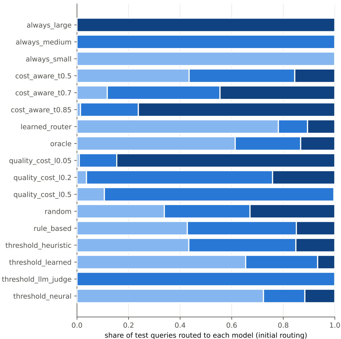
Model selection distribution
