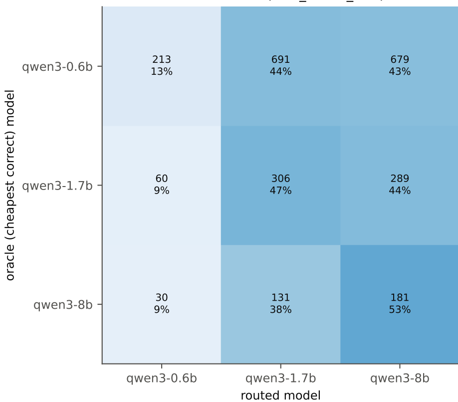
Router confusion matrix (cost_aware_t0.7)
