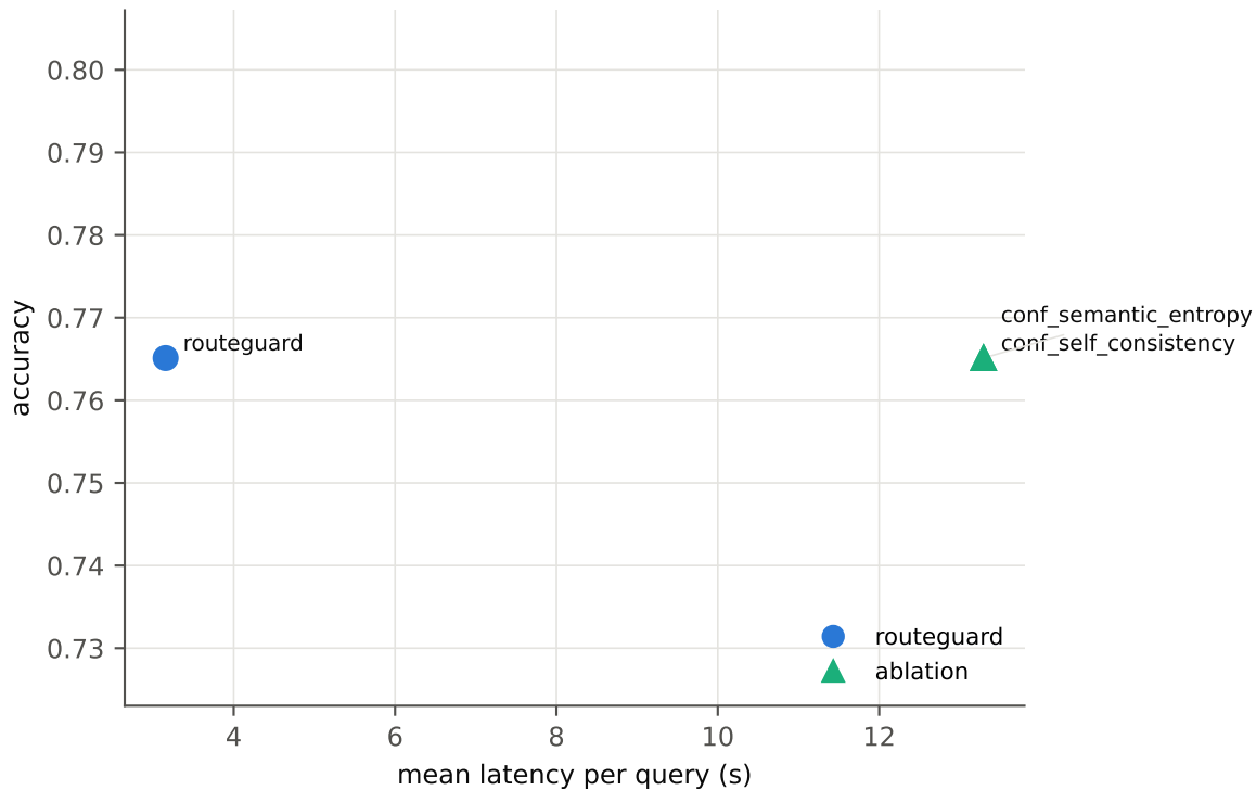
Quality vs latency
