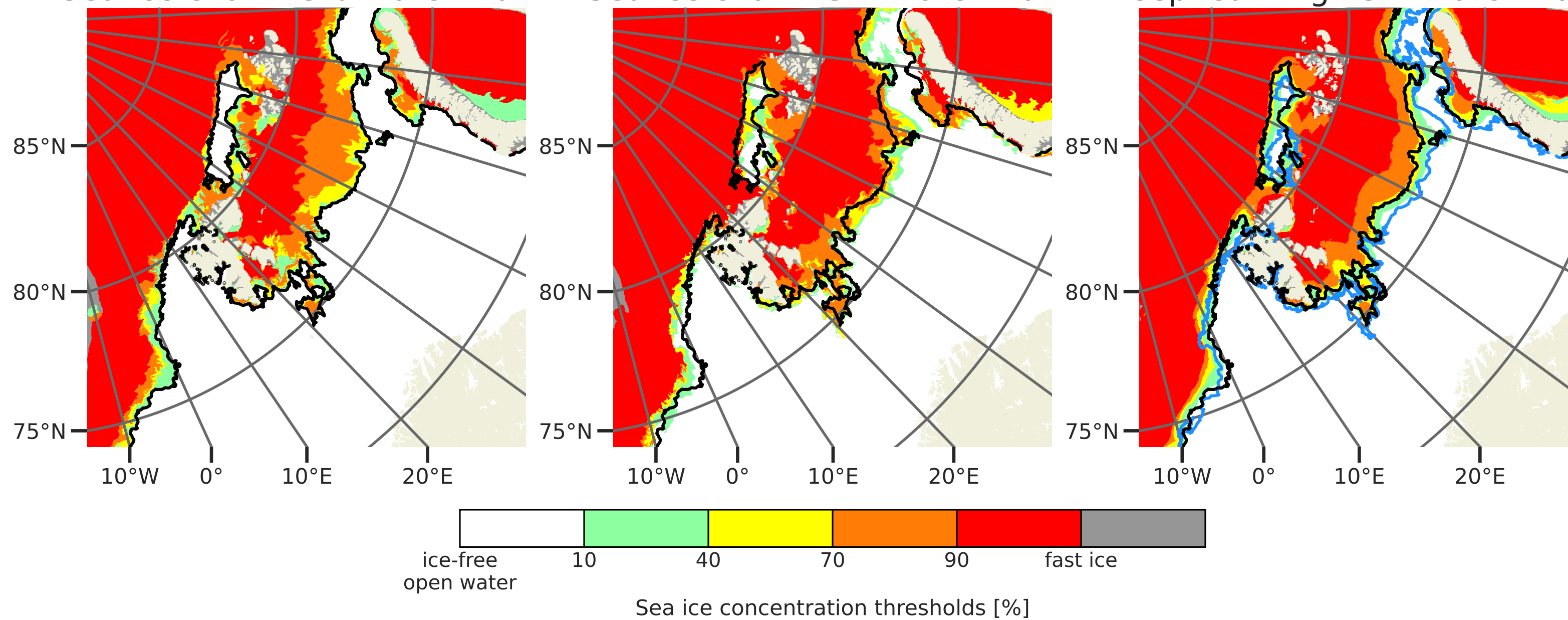
Sea ice chart 23rd March 2022
