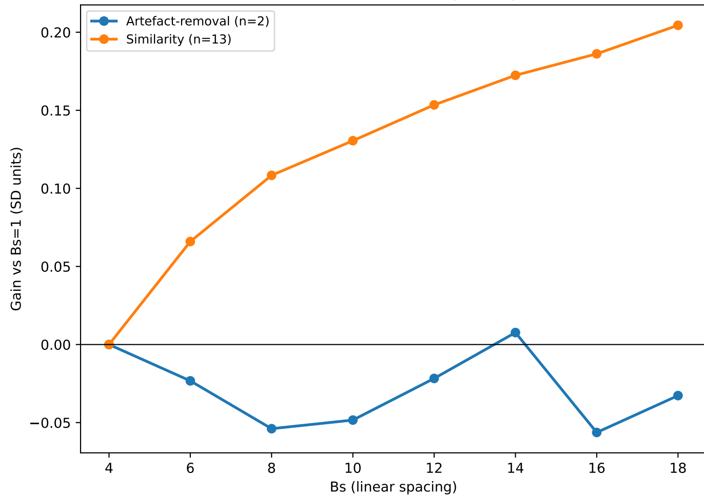
Metric families read separately
