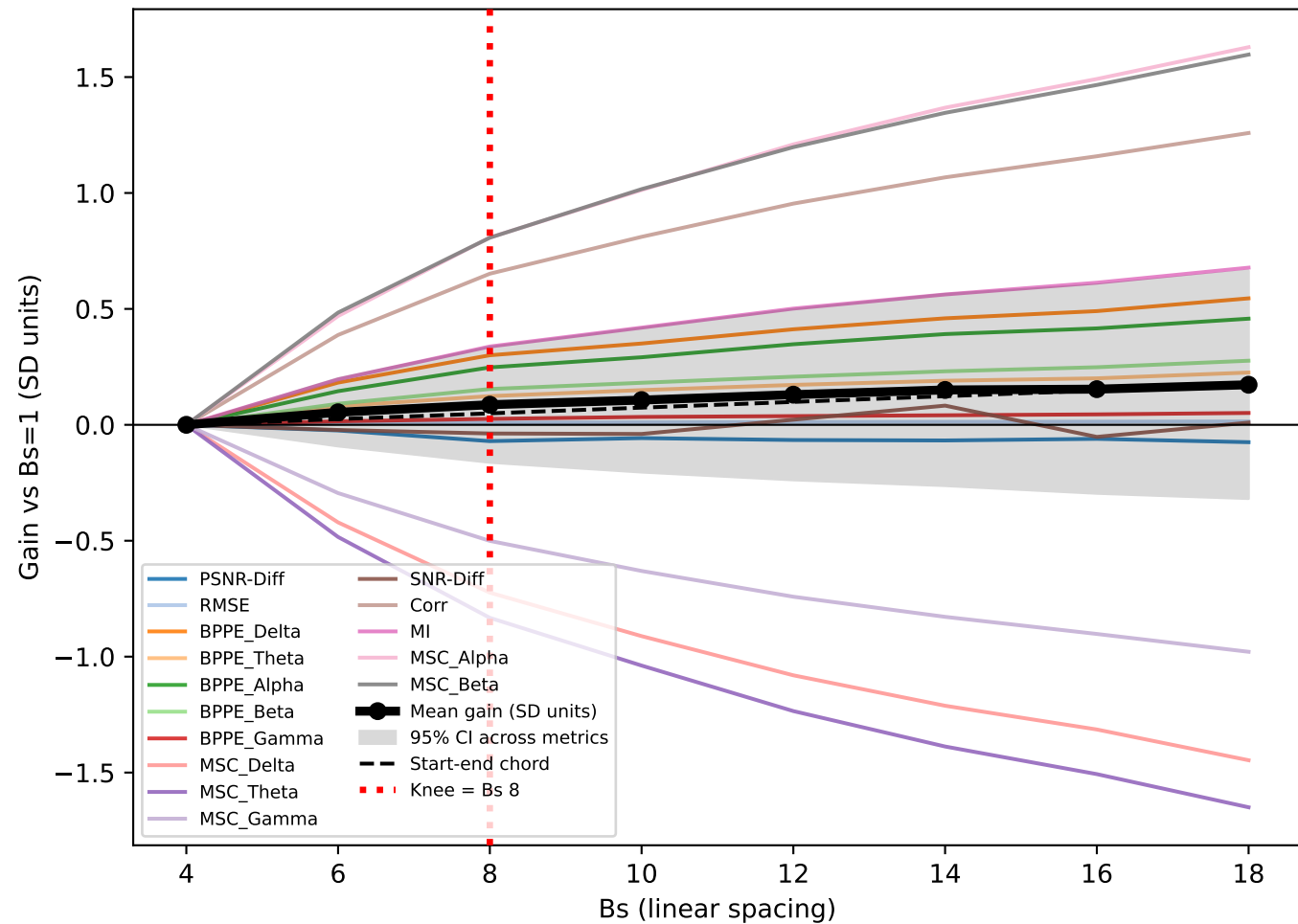
Lower Bound X v2 (Kneedle - linear): All Individual Metrics
