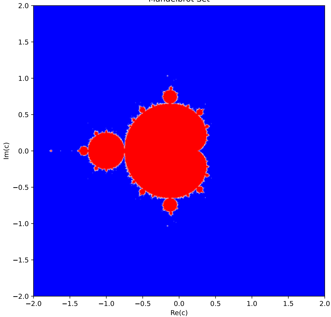
Mandelbrot Set
