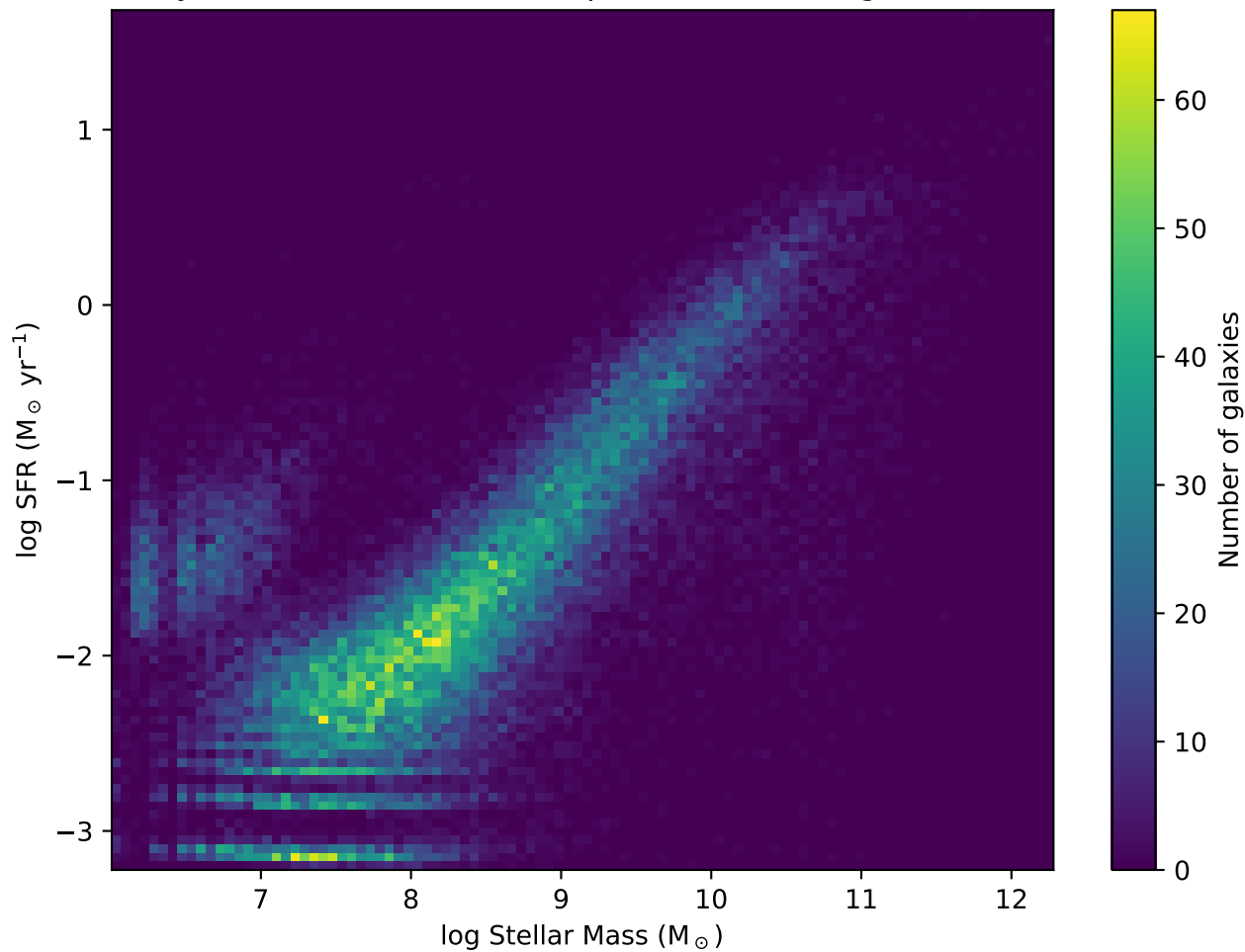
Galaxy Star Formation Main Sequence - 2D Histogram (EAGLE)
