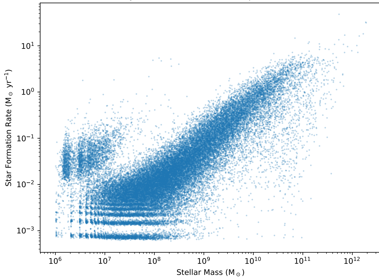
Galaxy Star Formation Main Sequence (EAGLE)
