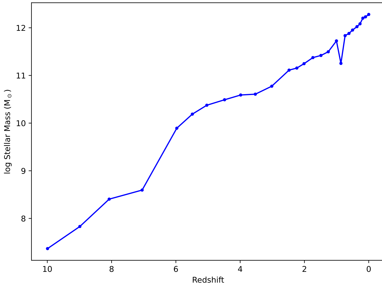
Main Branch of Most Massive Galaxy
