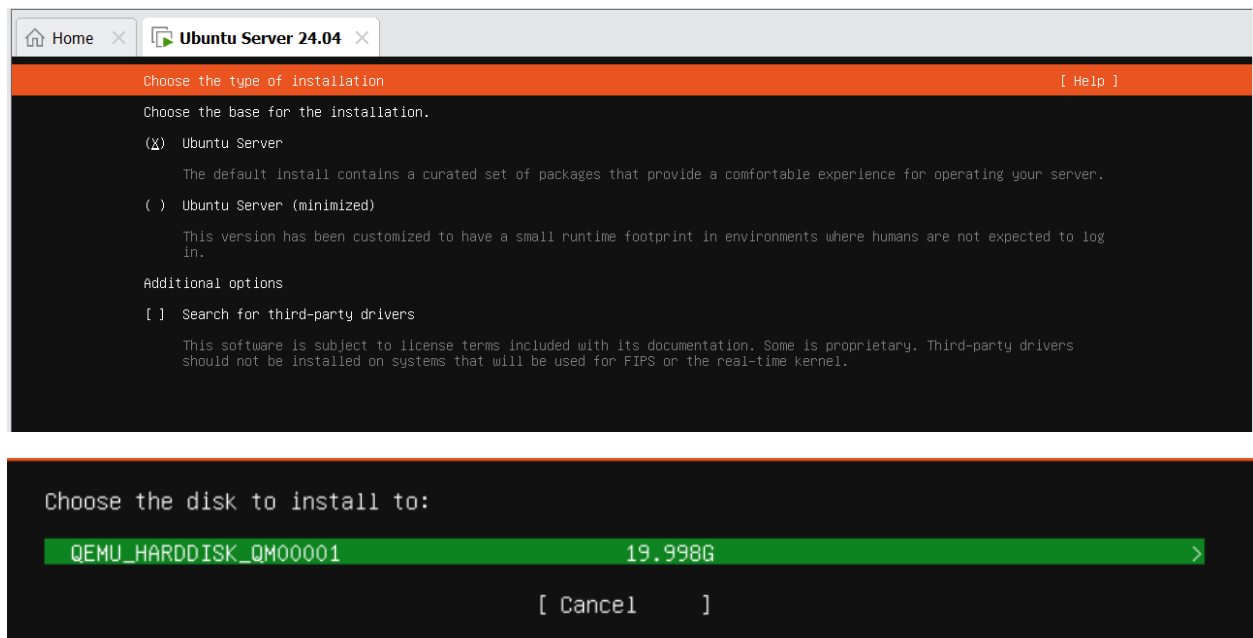
Caption: Task 10 - Selection of the virtual hard disk for Ubuntu Server installation.
