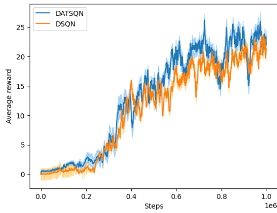
Figure 9. Average reward achieved by each RL agent across 3 different seeds in the Road Runner environment.
