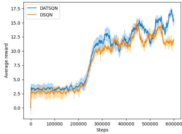
Figure 10. Average reward achieved by each RL agent across 3 different seeds in the Beam Rider environment.
