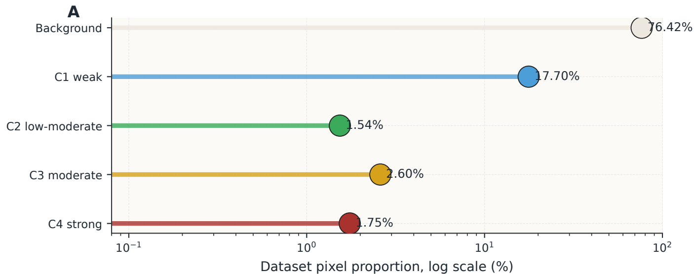
Ordinal class
