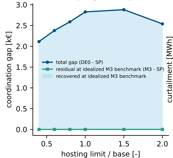
Gap vs grid scarcity
