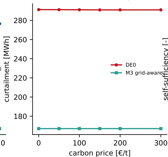
Curtailment vs carbon price
