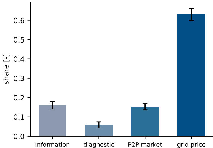
Mechanism shares (mean \pm s.d.)
