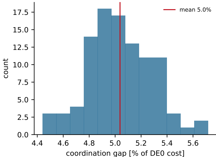
Gap distribution across seeds
