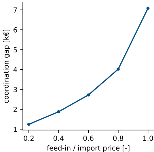
Gap vs feed-in price
