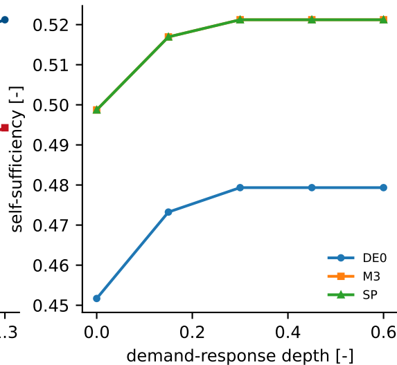
Self-sufficiency vs DR depth
