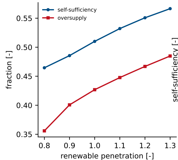
Self-sufficiency and oversupply vs RES
