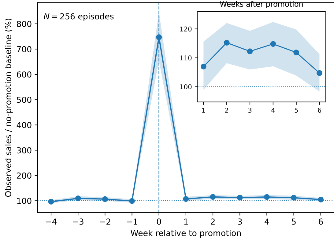
(b) Sales relative to no-promotion baseline
