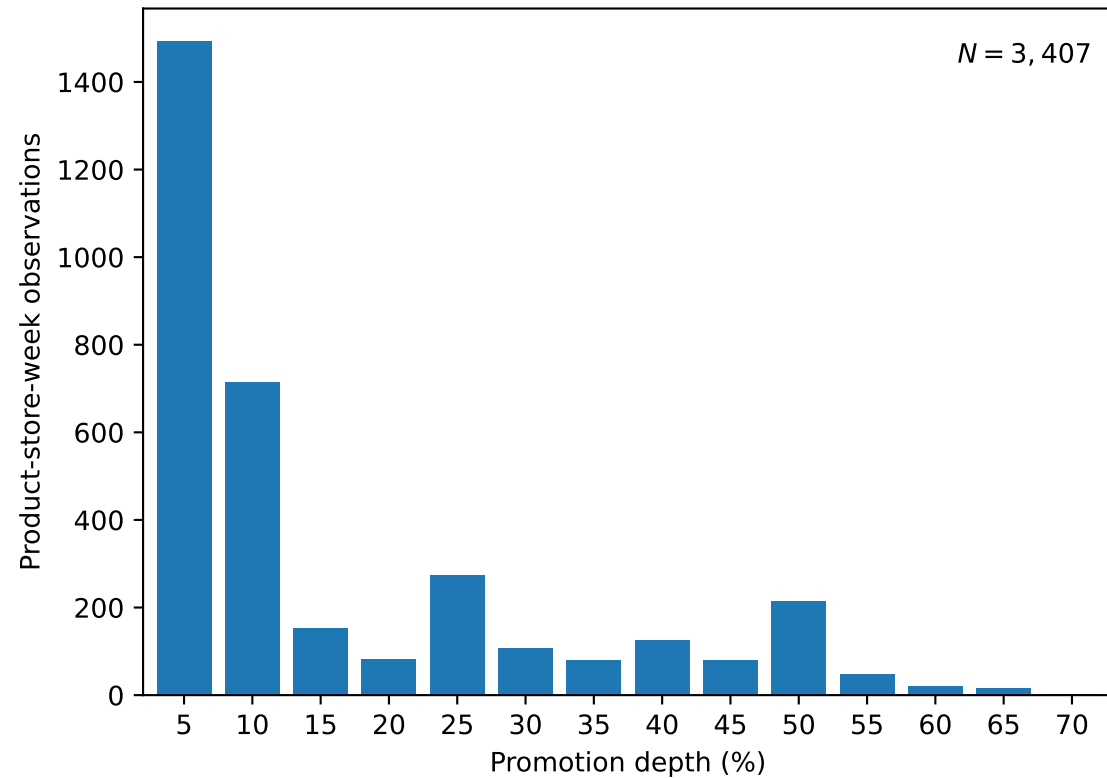
(a) Observed promotion depths
