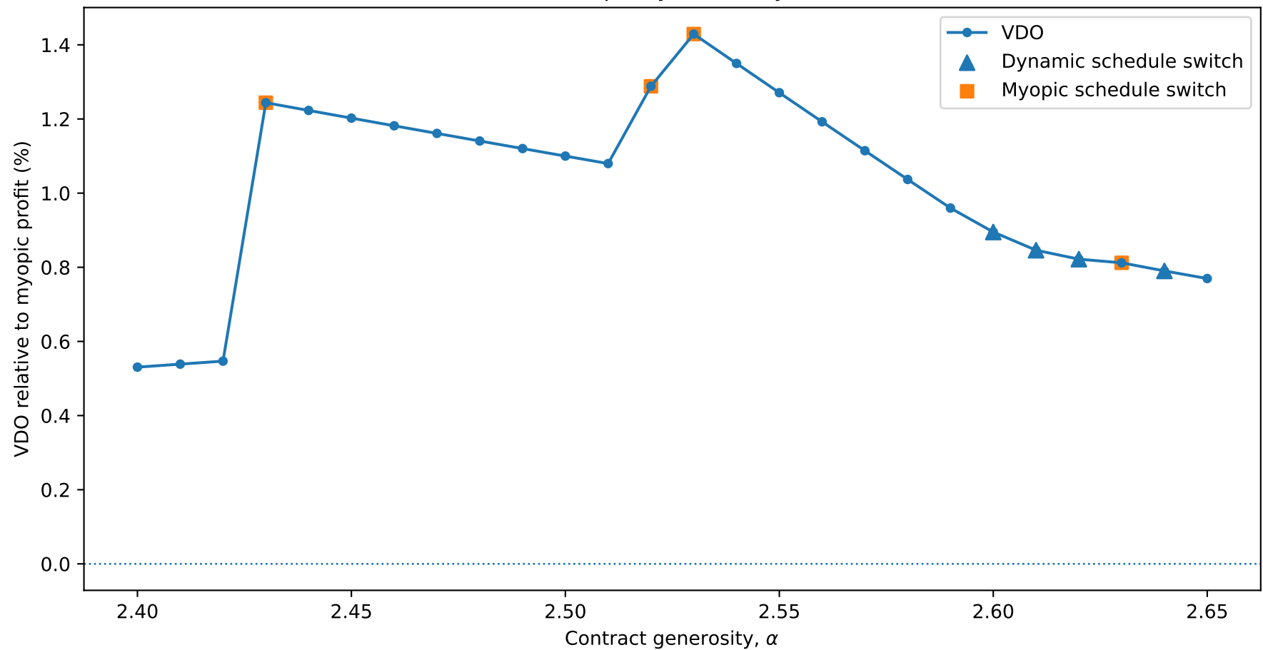
Local validation of the policy-boundary mechanism (B=2)
