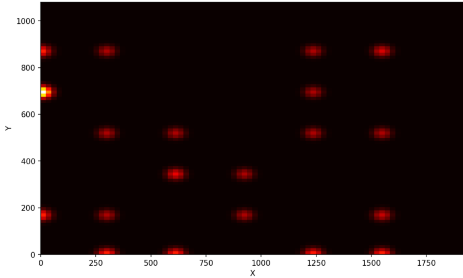
Gaze heatmap
