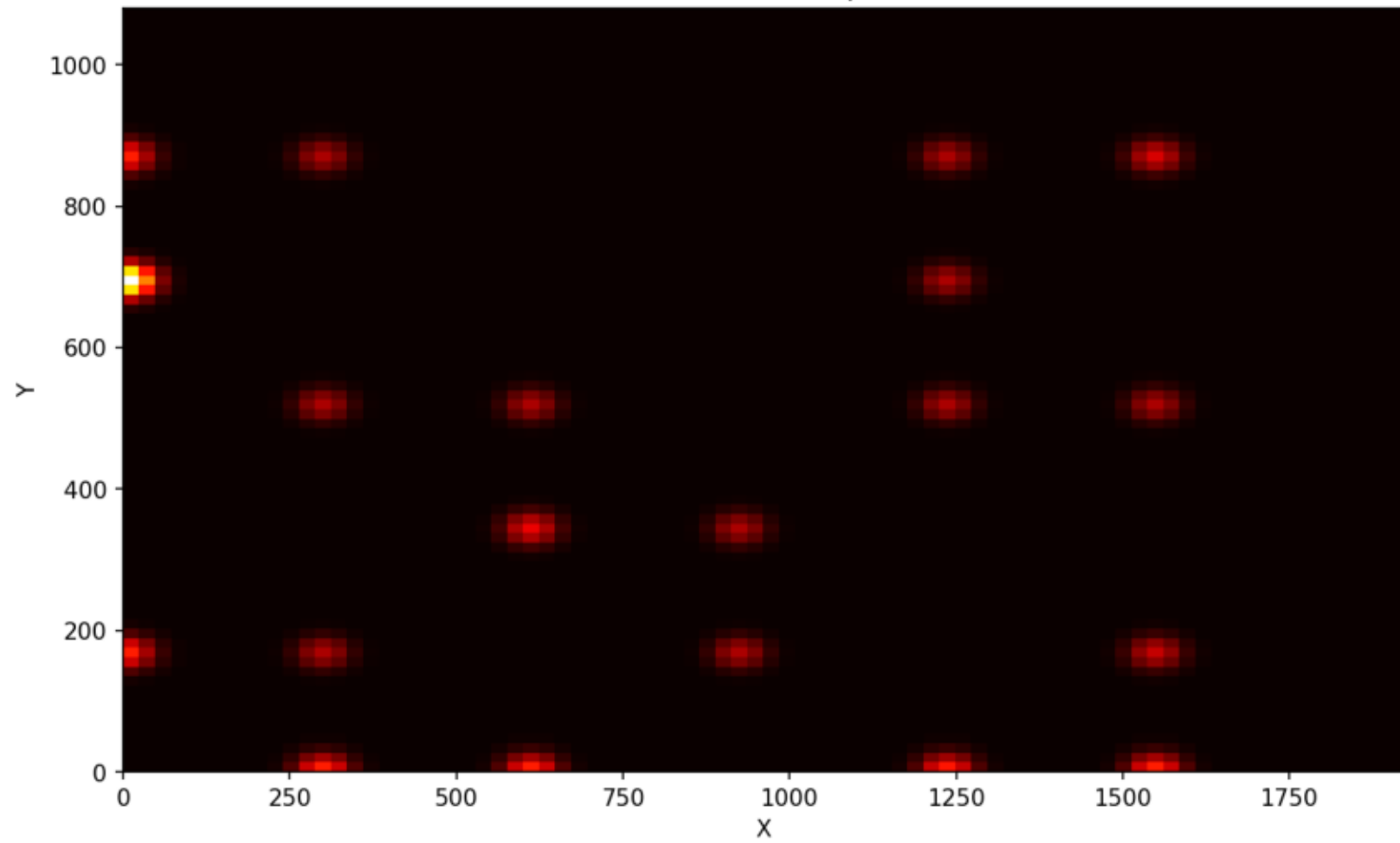
Gaze heatmap
