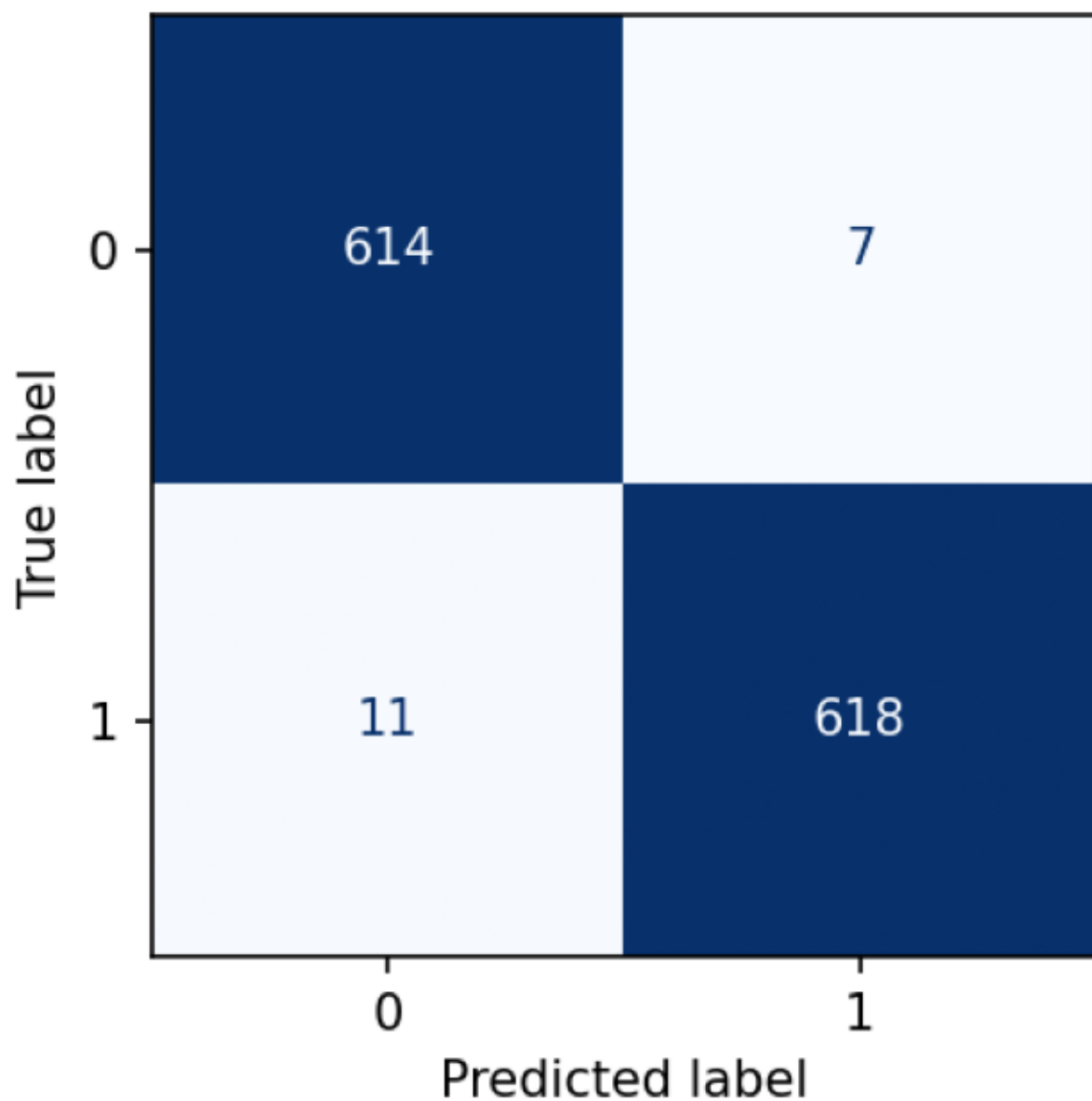
Decision Tree Confusion Matrix
