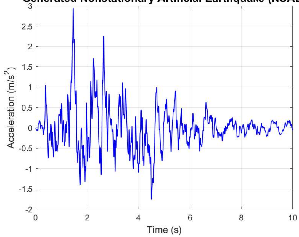
Generated Nonstationary Artificial Earthquake (NSAE)
