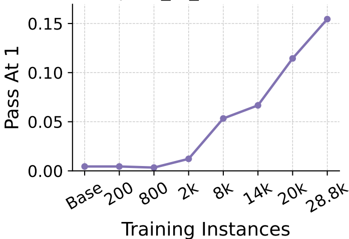
pass_at_1 vs Scale
