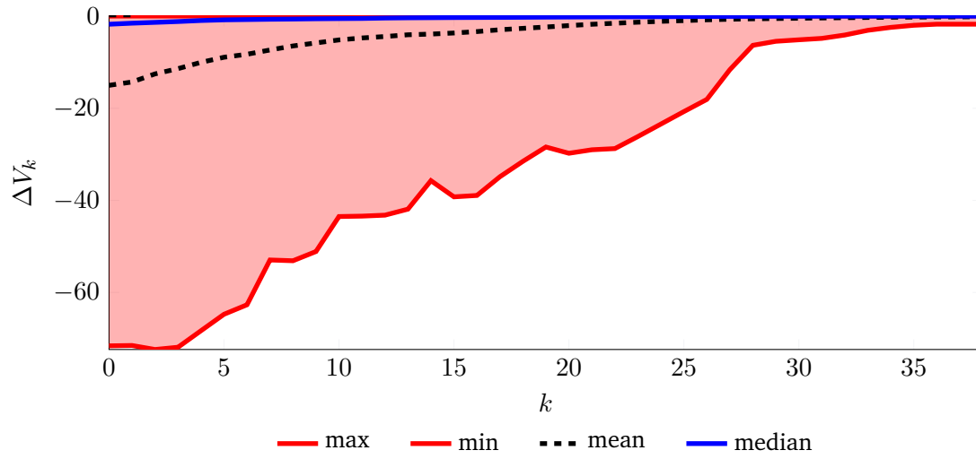
Figure 6.1: Double integrator cost descent. \Delta V = V_N(x_{k+1}) - V_N(x_k)
