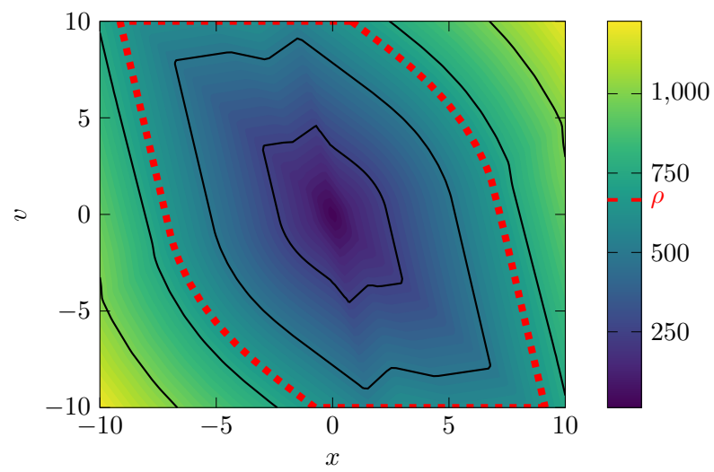
Figure 6.3: Double integrator Lyapunov landscape and ROA: 665.66
