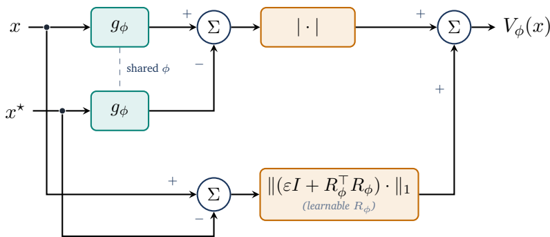
Figure 5.2: The neural Lyapunov architecture.
