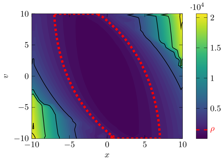
Figure 6.2: Double integrator Lyapunov landscape of the MPC optimal value function with an estimated ROA: 1.45e + 03 .
