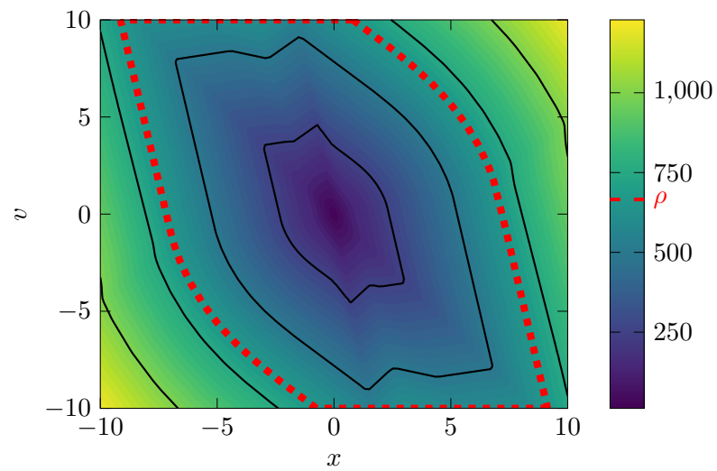
Figure 6.3: Double integrator Lyapunov landscape and ROA: 665.66
