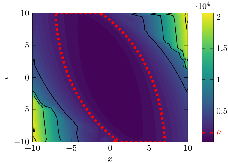
Figure 6.1: Double integrator Lyapunov landscape of the MPC optimal value function with an estimated ROA: 1.45e + 03 .
