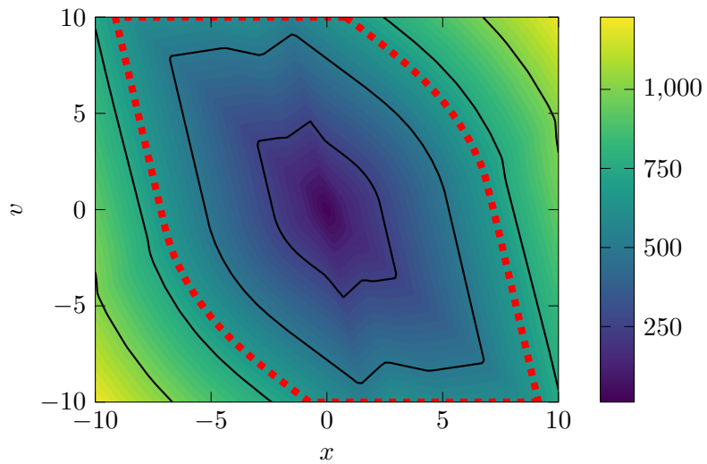
Figure 7.3: Double integrator Lyapunov landscape and ROA: value
