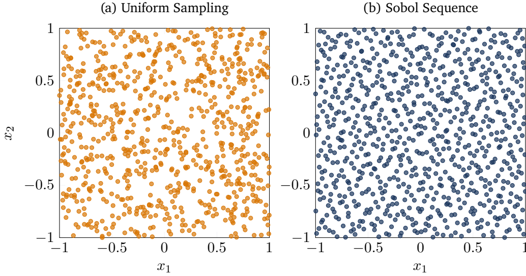
Figure 6.4: Comparisson of Sobol and uniform sampling in two dimensions.
