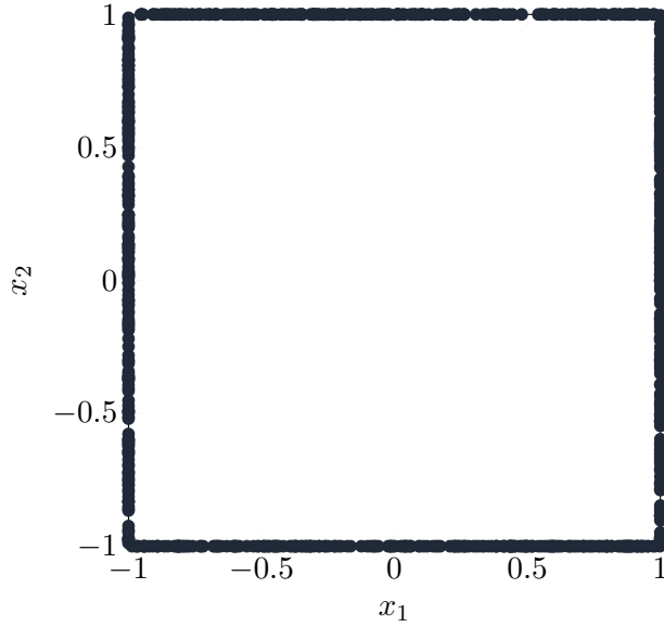
Figure 6.6: Visualization for boundary sampling of a 2 dimensional example.
