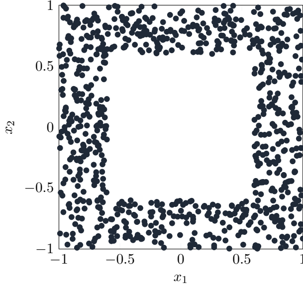
Figure 6.3: Illustration of uniformly drawn samples in the shell batch \mathcal{B}_{\text{ROA}} with \xi = 0.6 .
