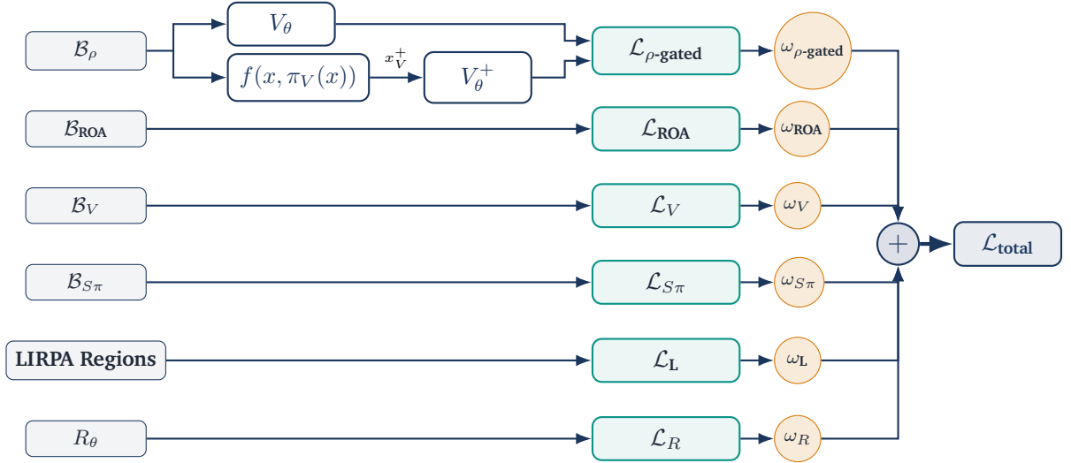
Figure 6.5: Loss flow visualization.
