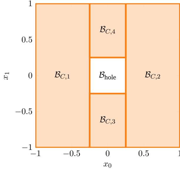
Figure 6.7: 2D Hole exclusion example with \mathcal{B}_{\text{hole}} := \{x \in \mathbb{R}^2 \mid \|x\|_{\infty} < 0.25\} .
