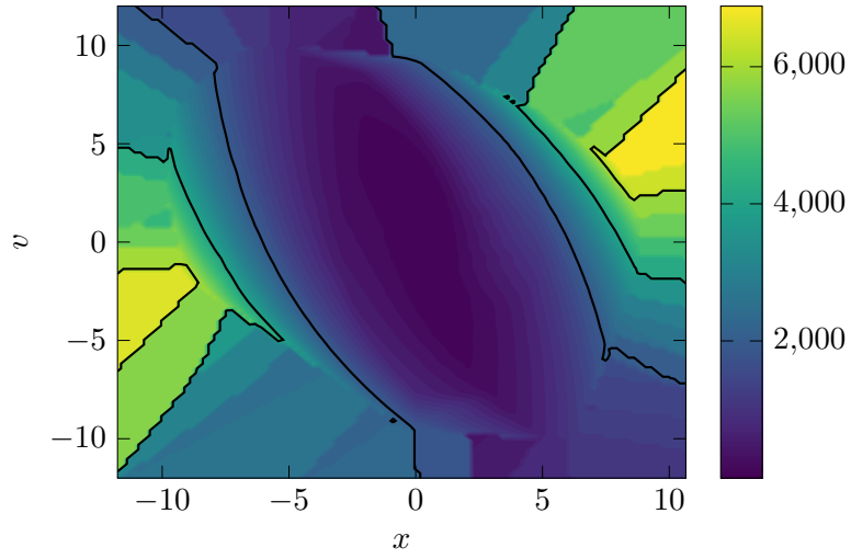
Figure 7.2: Double integrator Lyapunov landscape of the MPC optimal value function.
