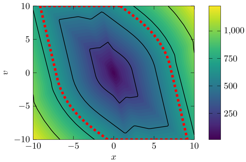
Figure 7.3: Double integrator Lyapunov landscape and ROA: value
