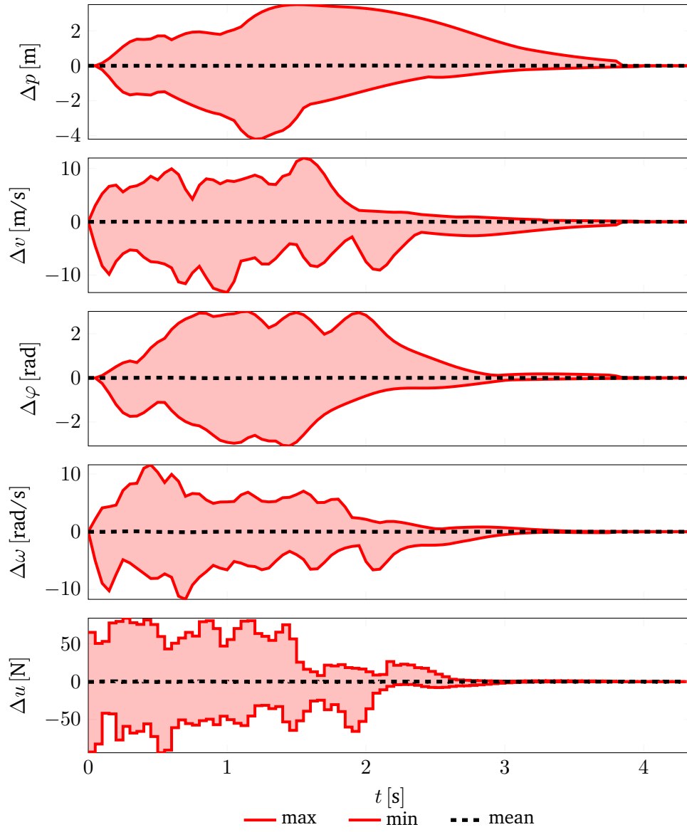
Figure 6.5: Cartpole error band. x_\theta - x_{\text{MPC}}
