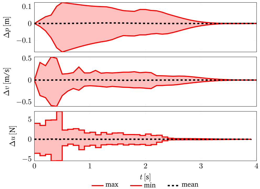
Figure 6.2: Closed-loop trajectory tracking error between the learned policy and the MPC expert for the double integrator.
