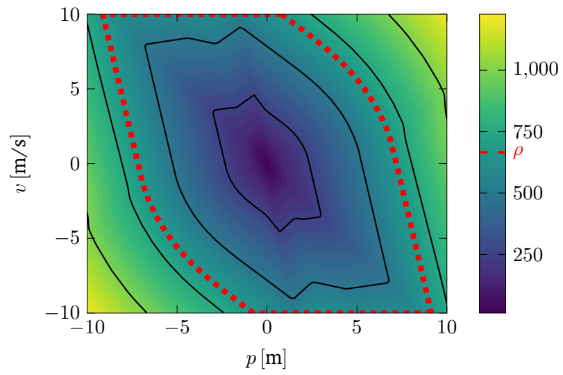
Figure 6.4: Learned Lyapunov function landscape V_\phi for the double integrator with the maximal certified region of attraction boundary \mathcal{V}_{\rho^*} at \rho^* = 665.66 .
