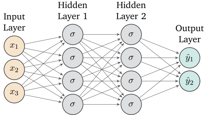
Figure 3.2: Architecture of an exemplary Multi-Layer Perceptron with three inputs, two outputs and two hidden layers with four neurons each. Illustration adapted from [19, Fig. 3.1]
