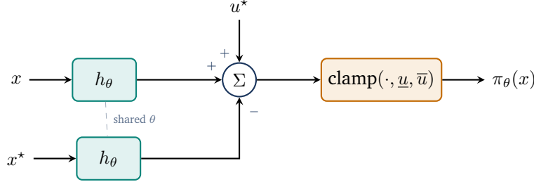
Figure 5.1: Architecture of the imitation control policy \pi_\theta(x) , which ensures exact control action replication at the equilibrium u_* and enforces hard control input constraints through clipping.
