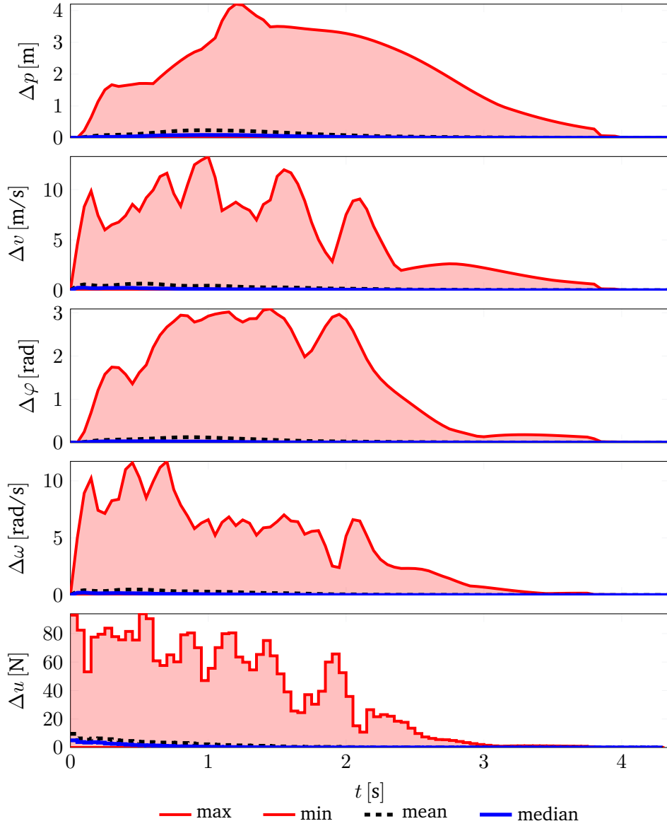
Figure 6.5: Closed-loop trajectory tracking error between the learned imitation policy and the MPC expert for the cartpole system, showing the error envelopes and the mean over time.
