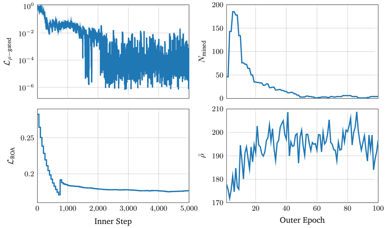
Figure 6.6: Co-training progression for the cartpole system, showing the gated condition loss \mathcal{L}_{\rho\text{-gated}} on the top left and the ROA loss \mathcal{L}_{\text{ROA}} on the bottom left over inner optimization steps, alongside the mined counterexamples N_{\text{mined}} on the top right and the estimated sublevel set bound \tilde{\rho} on the bottom right over outer epochs.
