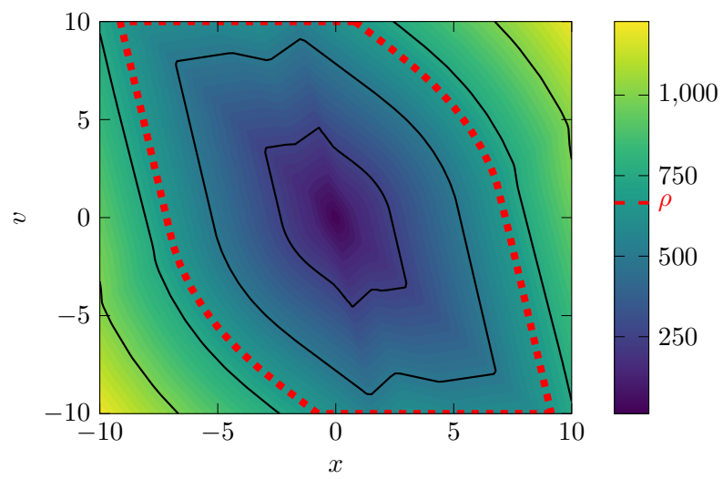
Figure 7.3: Double integrator Lyapunov landscape and ROA: 665.66
