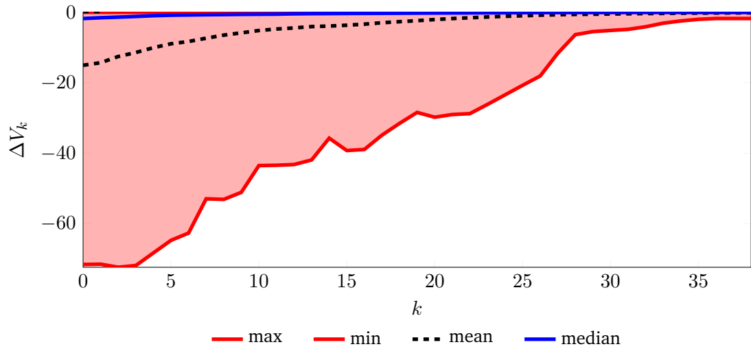
Figure 7.1: Double integrator cost descent. \Delta V = V_N(x_{k+1}) - V_N(x_k)
