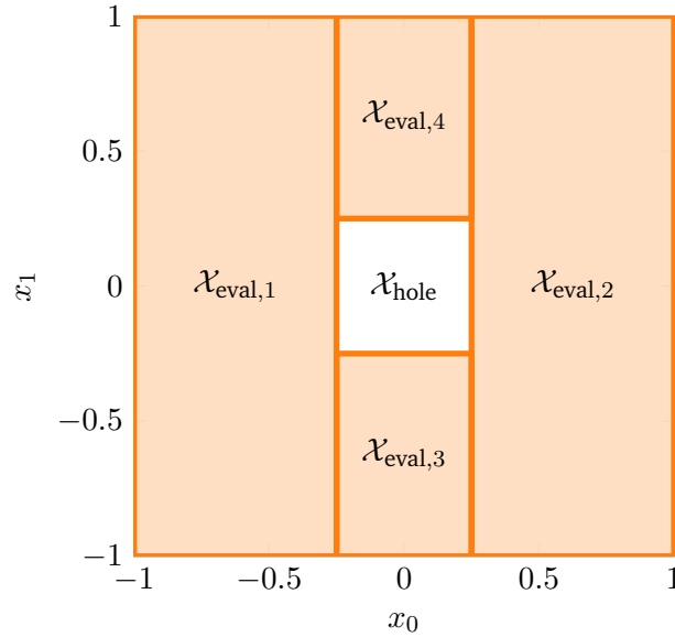
Figure 6.8: 2D Hole exclusion example with \mathcal{X}_{\text{hole}} := \{x \in \mathbb{R}^2 \mid \|x\|_\infty < 0.25\} .
