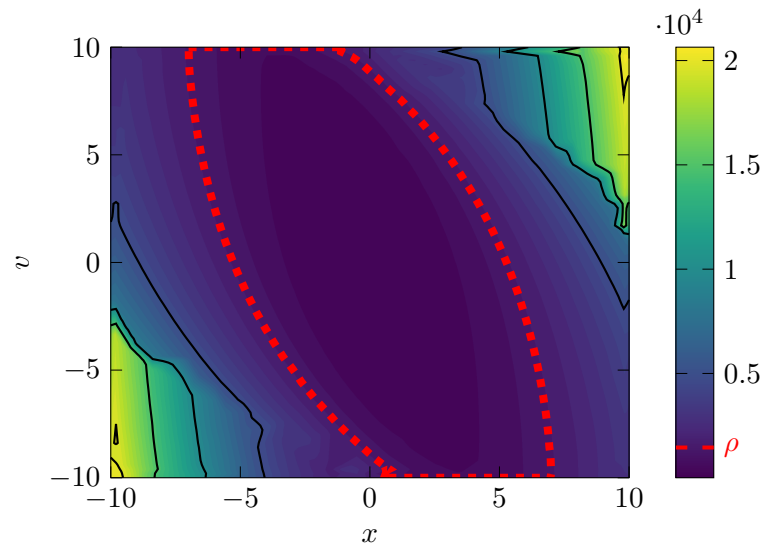
Figure 7.2: Double integrator Lyapunov landscape of the MPC optimal value function with an estimated ROA: 1.45e + 03 .
