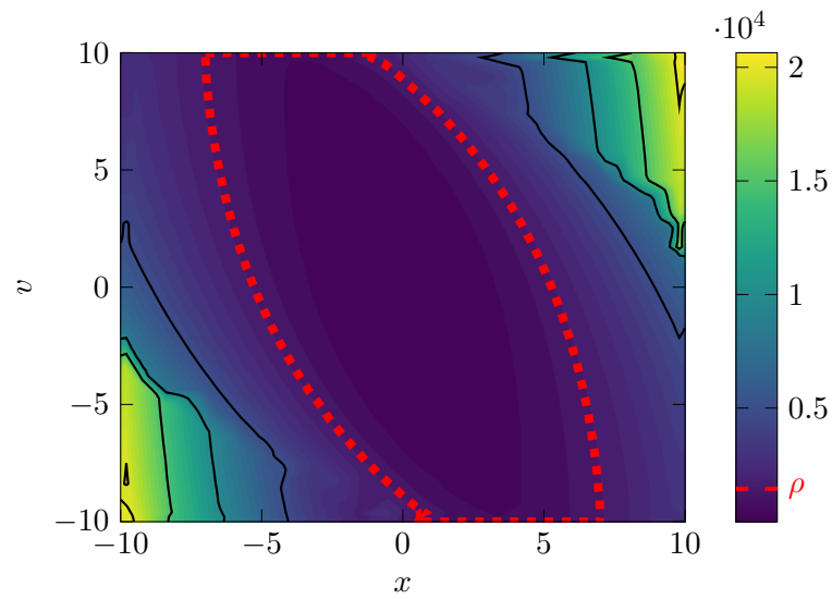
Figure 6.3: Double integrator Lyapunov landscape of the MPC optimal value function with an estimated ROA: 1.45e + 03 .
