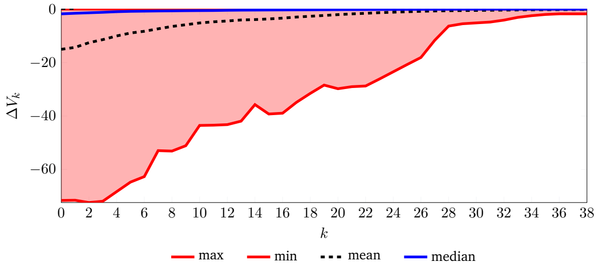
Figure 6.2: Double integrator cost descent \Delta V = V_N(x^+) - V_N(x) .
