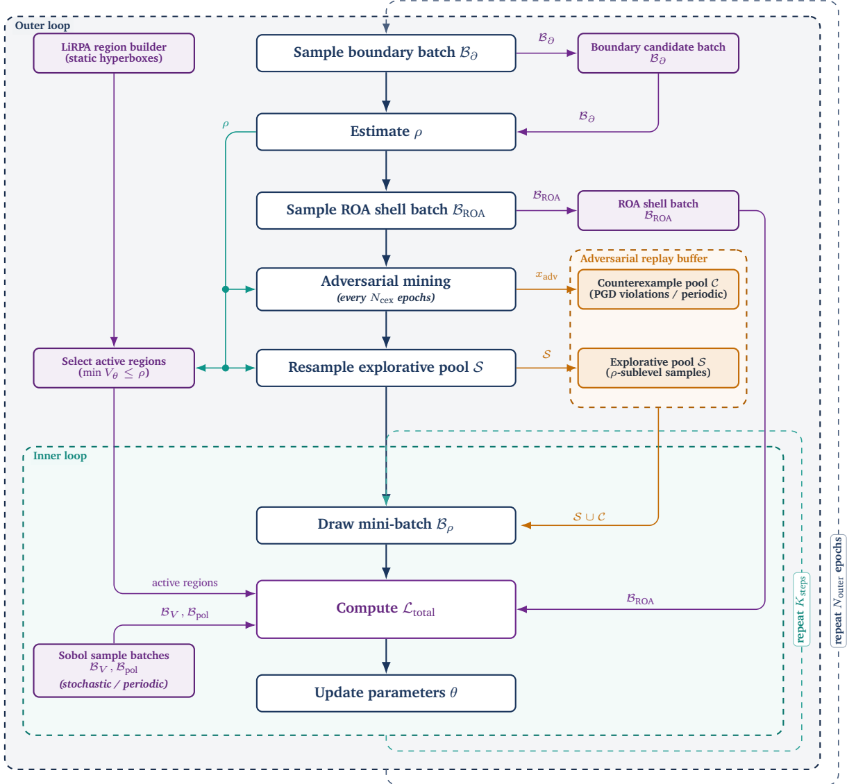
Figure 5.7: Overview of the falsification-guided training framework. The architecture is divided into an outer epoch-level loop responsible for state space exploration, boundary estimation, and adversarial mining, and an inner step-level loop that optimizes the network parameters based on the generated sample pools.
