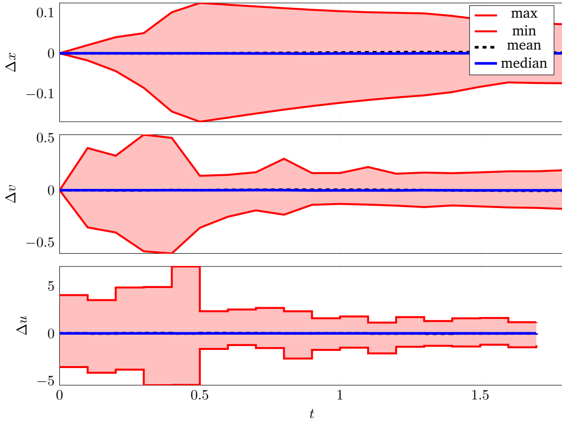
Figure 6.1: Double integrator error band. x_\theta - x_{\text{MPC}}
