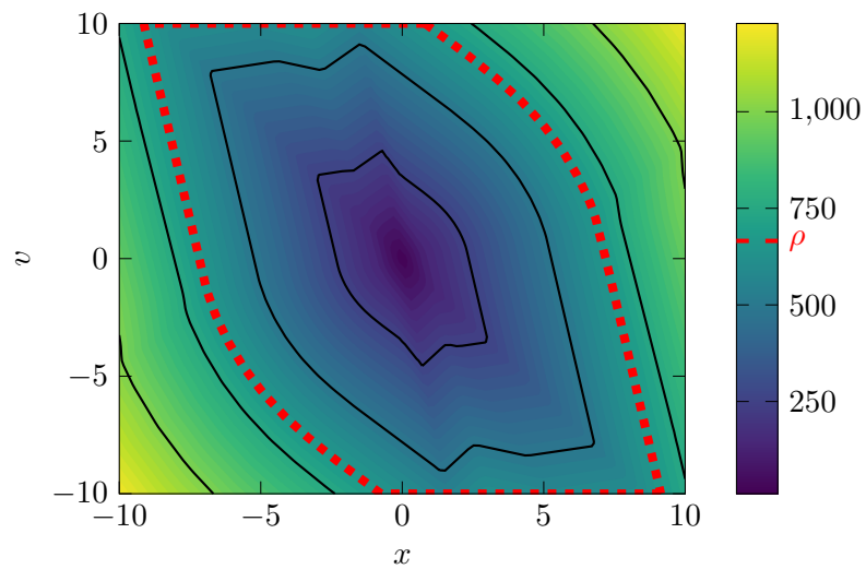
Figure 6.4: Double integrator Lyapunov landscape and ROA: 665.66
