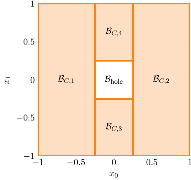
Figure 6.9: 2D Hole exclusion example with \mathcal{B}_{\text{hole}} := \{x \in \mathbb{R}^2 \mid \|x\|_\infty < 0.25\} .
