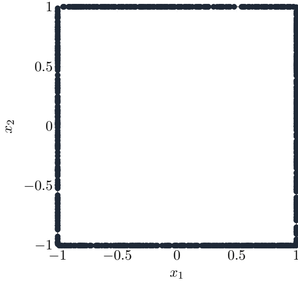
Figure 6.8: Visualization for boundary sampling of a 2 dimensional example.
