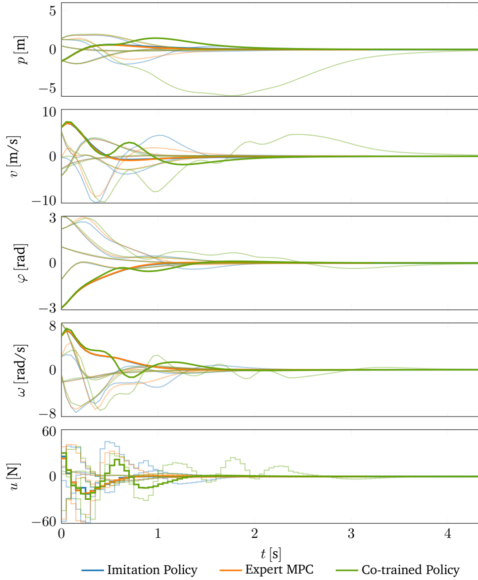
Figure A.3: Closed-loop state and control input trajectories comparing the learned imitation policy and the MPC expert for five initial states on the cartpole system.
