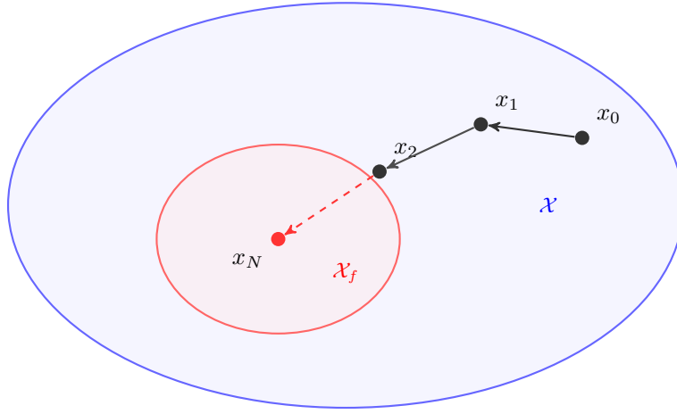
Figure 2.1: Predicted state trajectory x_0, \dots, x_N evolving within the state constraint set \mathcal{X} (blue) and terminating inside the terminal constraint set \mathcal{X}_f \subseteq \mathcal{X} (red).
