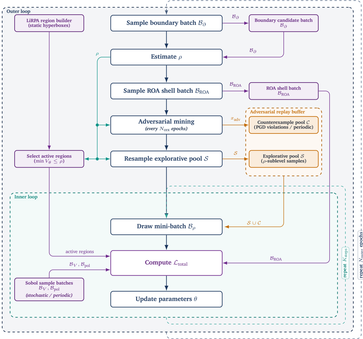
Figure 5.7: Overview of the falsification-guided co-training data flow, showing the outer epoch loop for boundary estimation, region selection, and adversarial mining into the replay buffer, alongside the inner optimization loop for neural network parameter updates.
