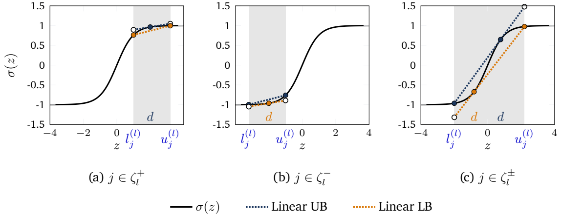
Figure 4.1: Linear bounds for general S-shaped activation functions \sigma(z) = \tanh(z) , inspired by Zhang et al. [9]. The navy dotted lines denote the upper bounds and the amber dotted lines denote the lower bounds.
