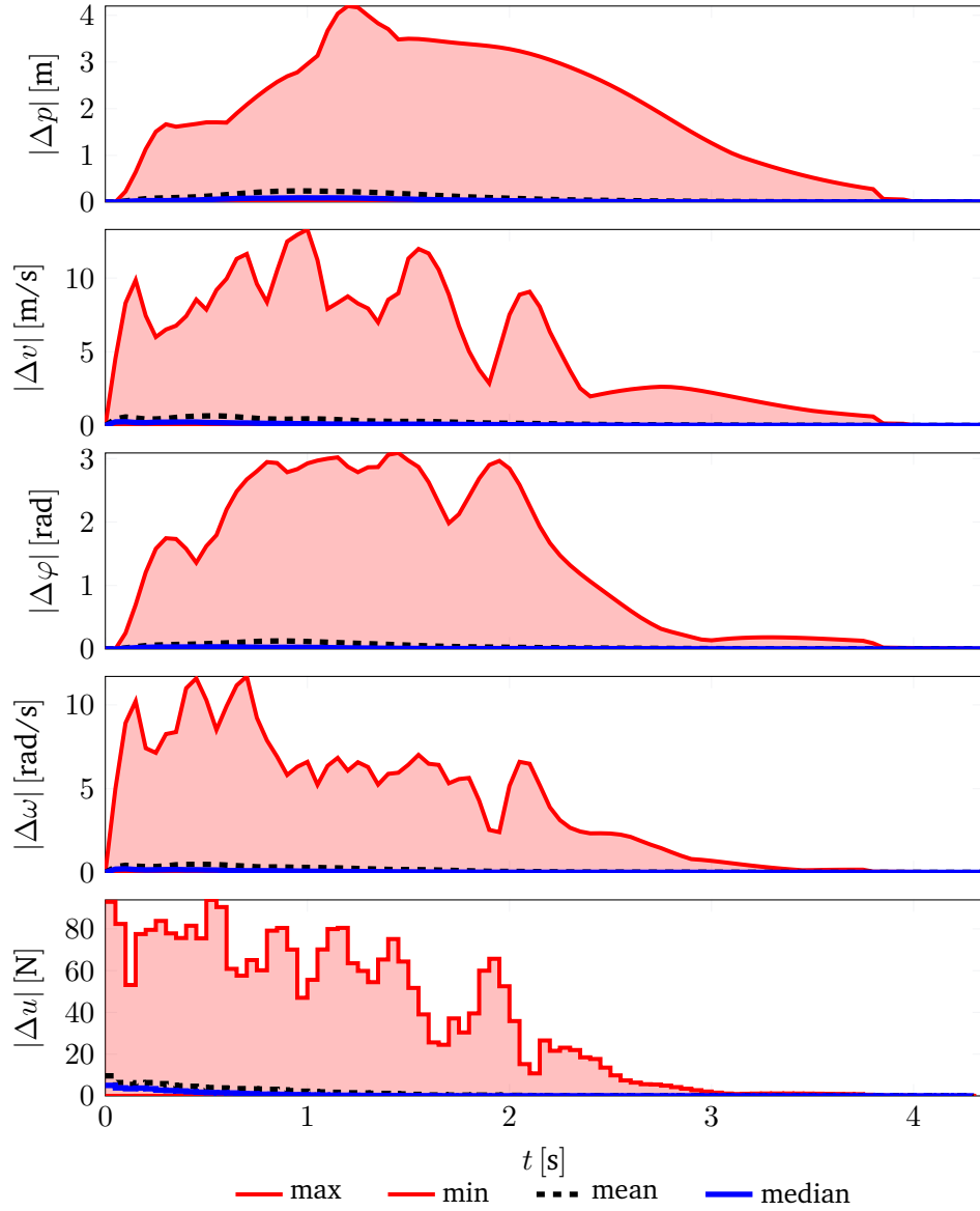
Figure 6.6: Closed-loop trajectory tracking error between the learned imitation policy and the MPC expert for the cartpole system, showing the error deviations, mean and median over time.
