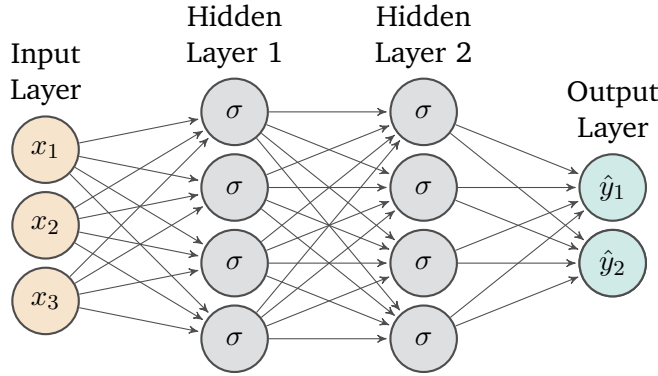
Figure 3.2: Architecture of an exemplary Multi-Layer Perceptron with three inputs x_1, \dots, x_3 , two outputs \hat{y}_1, \hat{y}_2 and two hidden layers L - 1 = 2 with four neurons each n_h = 4 . The illustration is adapted from [19, Fig. 3.1]
