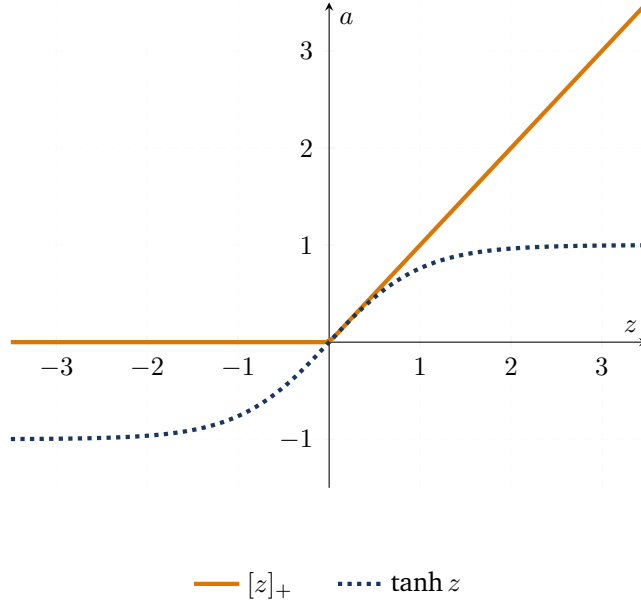
Figure 3.1: Standard activation functions \tanh and ReLU for neural control policies, where z denotes the pre-activation and a = \sigma(z) denotes the activation value.
