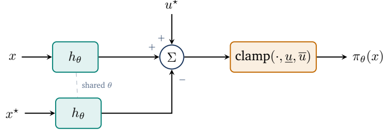
Figure 5.1: Architecture of the imitation control policy \pi_\theta(x) , which ensures exact control action replication at the equilibrium u_\star and enforces hard control input constraints through clipping.
